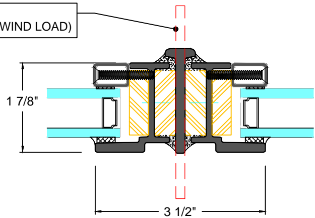
H TYPICAL JOINING MULLION
