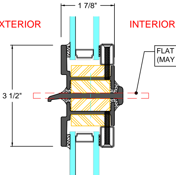
G TYPICAL STACKING MULLION
