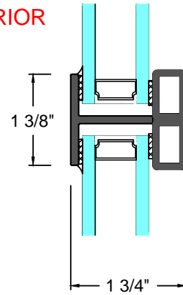
F TYPICAL HORIZONTAL MUNTIN
