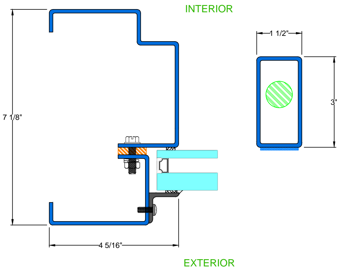
A&B — TYPICAL FIXED JAMB
