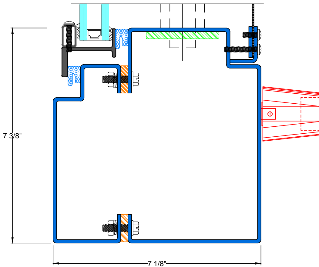
H TYPICAL SILL
