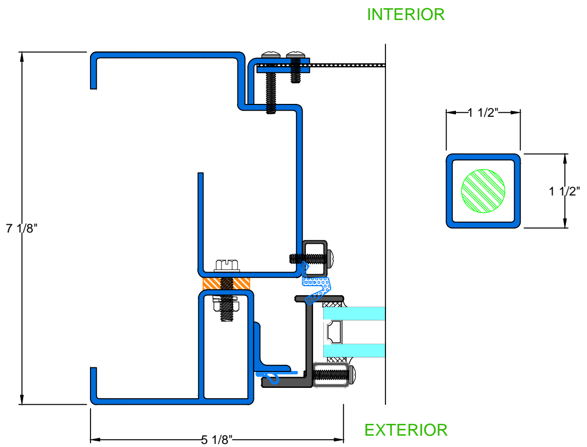
C&D TYPICAL OPERABLE JAMB
