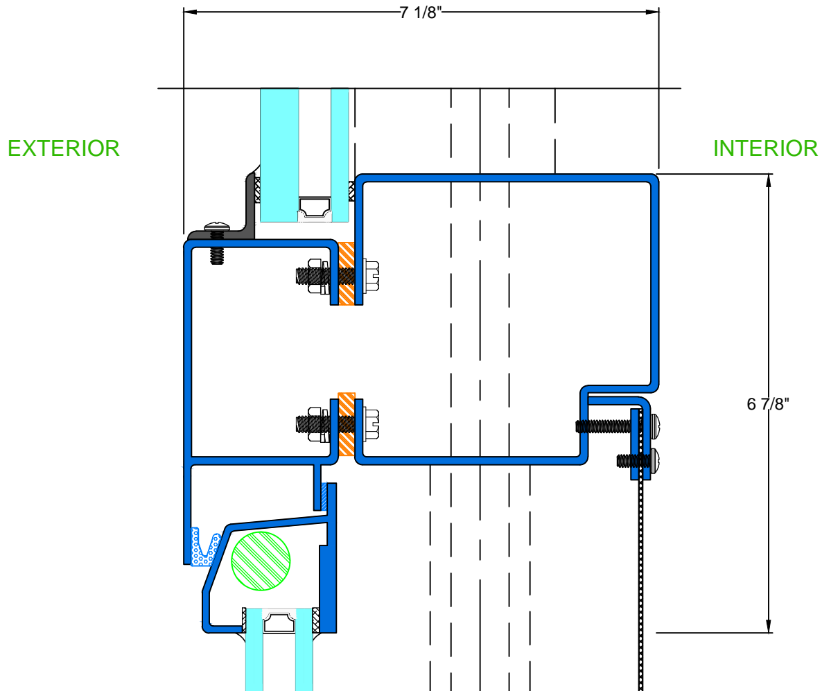
F TYPICAL MULLION
