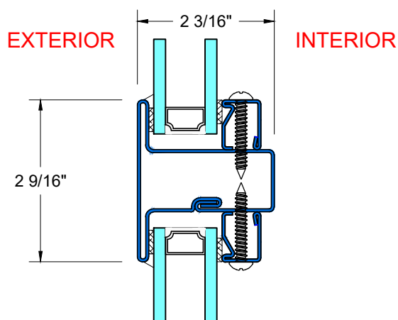
D TYPICAL MUNTIN
