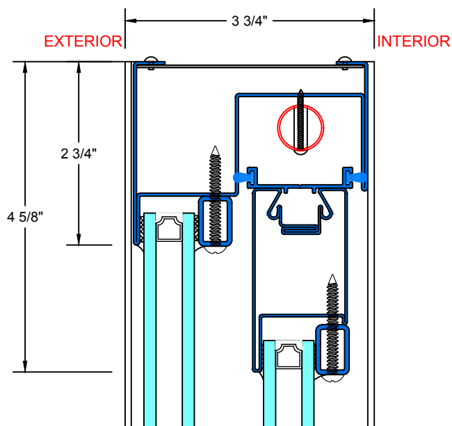
TYPICAL RIGHT JAMB
