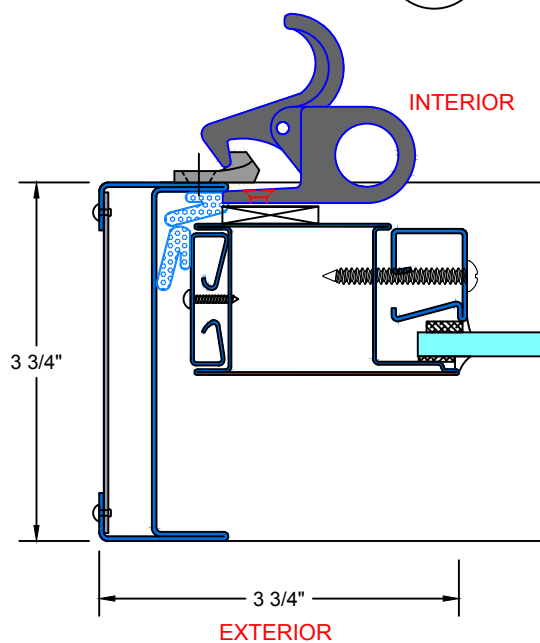
1 TYPICAL LEFT JAMB W/ 1/4" GLASS
