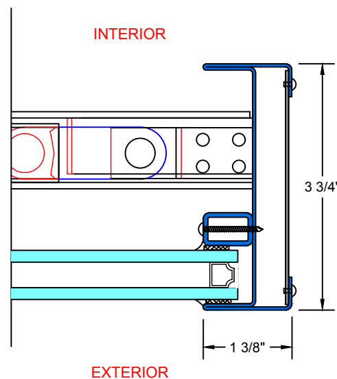
TYPICAL RIGHT JAMB
