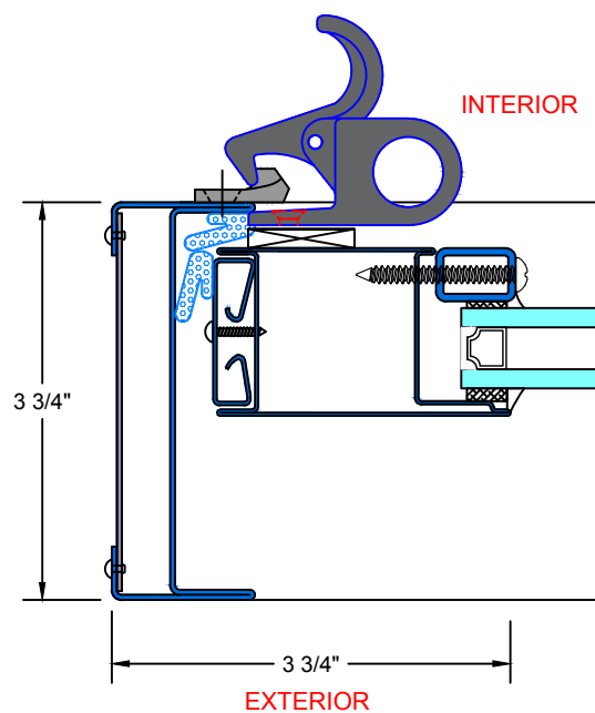
2 TYPICAL LEFT JAMB W/ 3/4" GLASS
