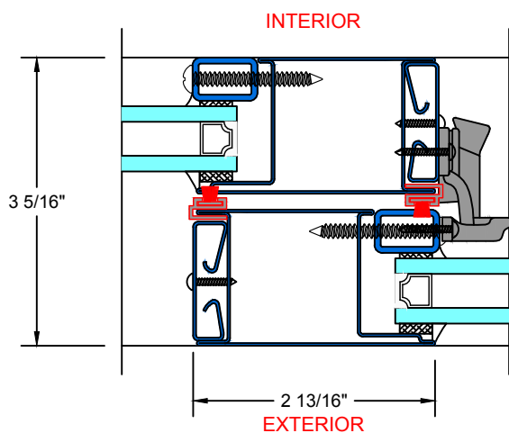
TYPICAL MEETING RAIL
