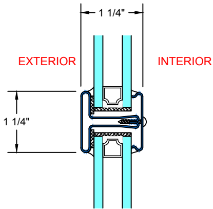
K TYPICAL HORIZONTAL MUNTIN
