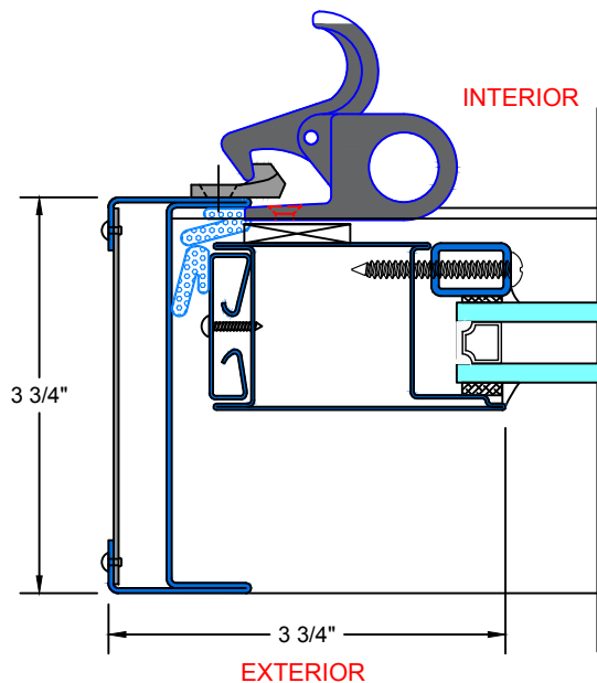
TYPICAL LEFT JAMB
