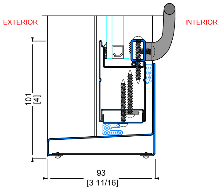
G TYPICAL SILL
