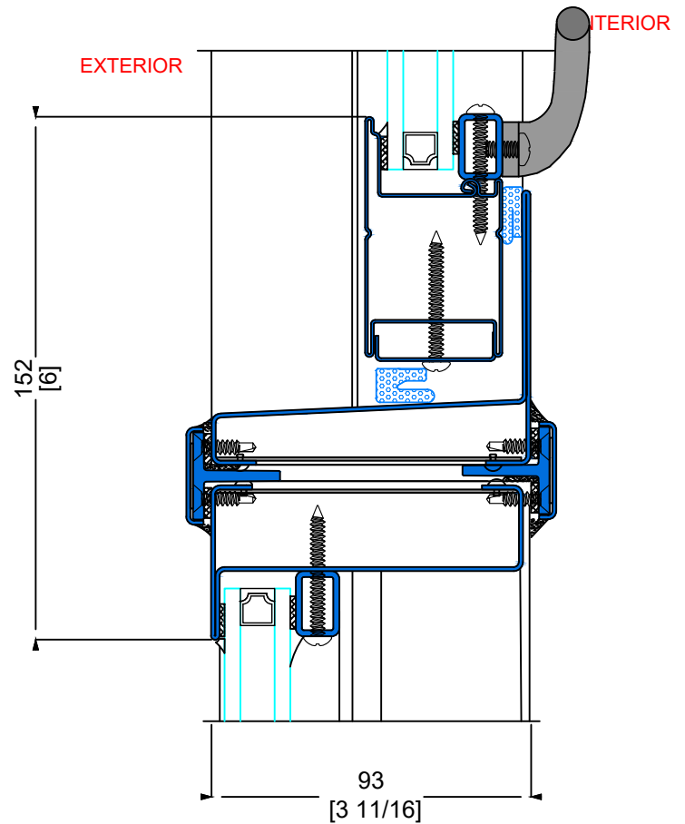
Q TYPICAL STACKING MULLION W/ TRANSOM BELOW
