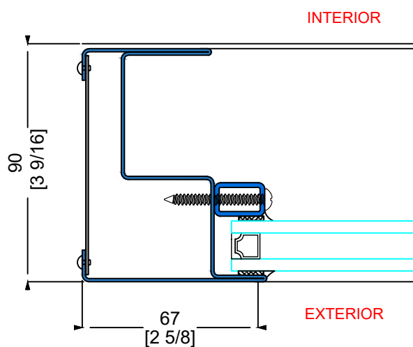
H&I TYPICAL TRANSOM JAMB
