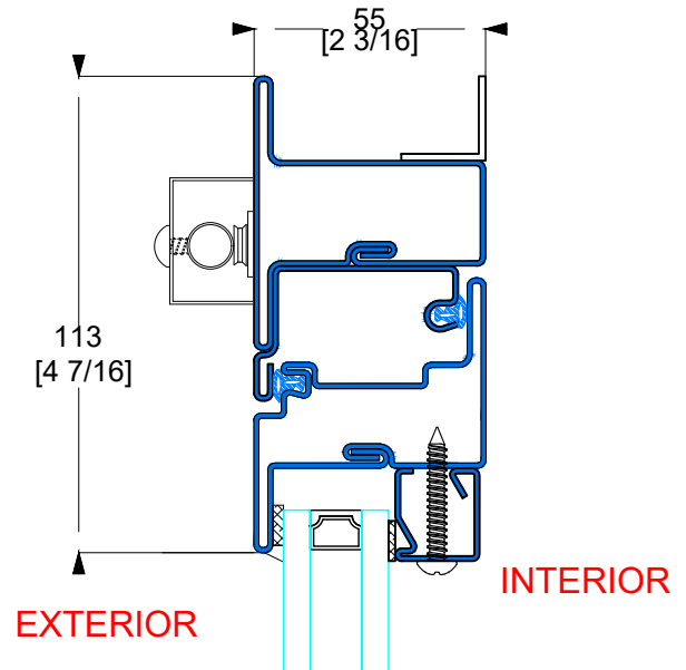
P TYPICAL STACKING HEAD
