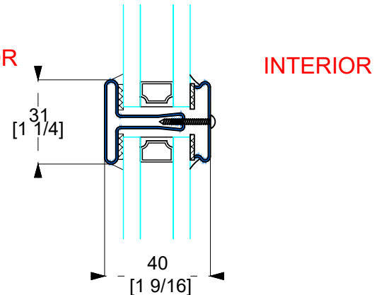
K&L TYPICAL HORIZONTAL MUNTIN W/ 1" GLASS
