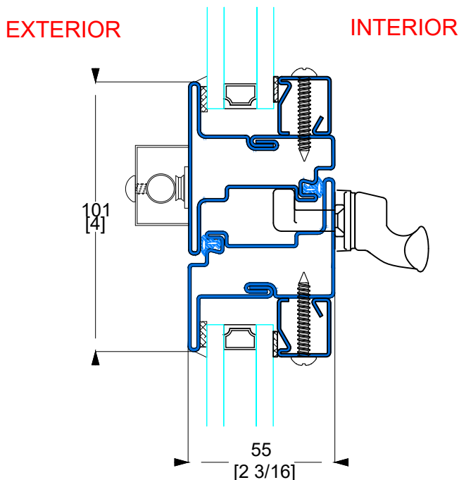
R TYPICAL STACKING MULLION
