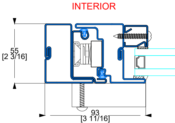
M&N TYPICAL STACKING JAMB
