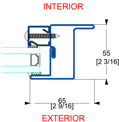
3 TYPICAL FIXED INTERIOR FLANGE
