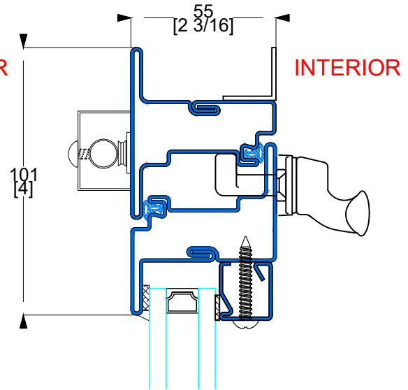
C TYPICAL HEAD
