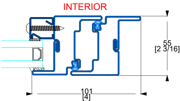
1 TYPICAL JAMB INTERIOR FLANGE
