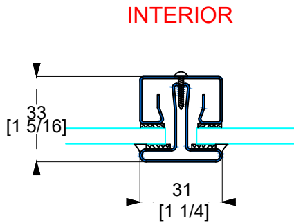
F TYPICAL VERTICAL MUNTIN W/ 1/4" GLASS
