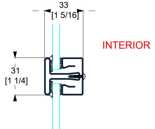
G TYPICAL HORIZONTAL MUNTIN W/ 1/4" GLASS
