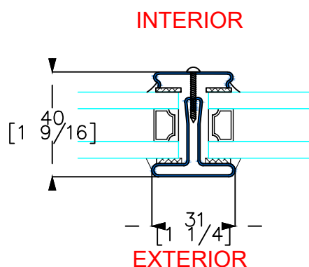
H&J TYPICAL VERTICAL MUNTIN W/ 1" GLASS
