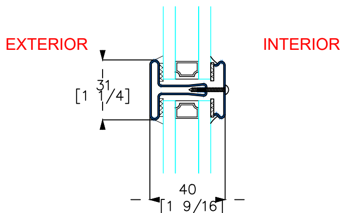
K&L TYPICAL HORIZONTAL MUNTIN W/ 1" GLASS
