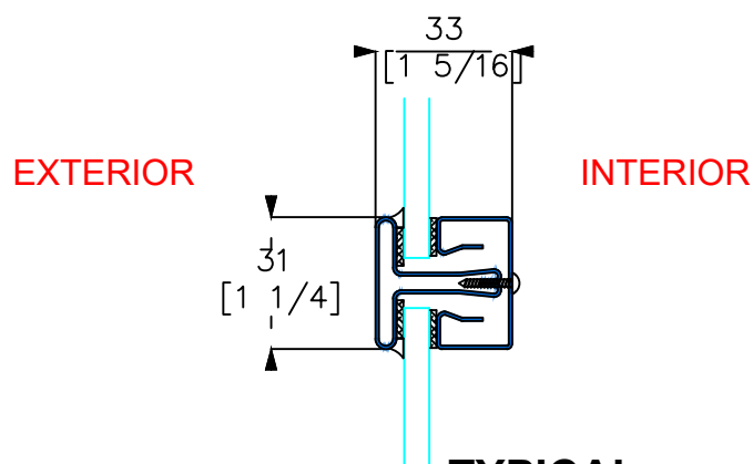
G TYPICAL HORIZONTAL MUNTIN W/ 1/4" GLASS
