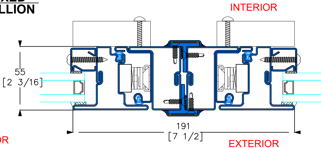
V TYPICAL OPERABLE JOINING MULLION
