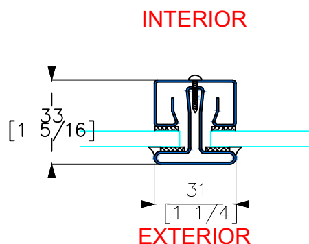
F TYPICAL VERTICAL MUNTIN W/ 1/4" GLASS
