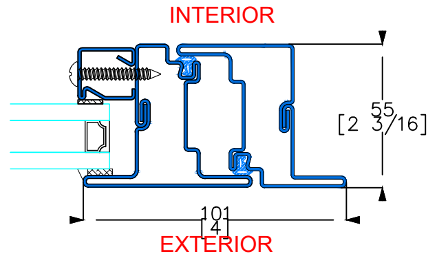
2 TYPICAL JAMB EXTERIOR FLANGE
