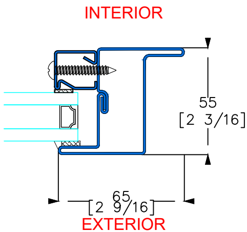
3 TYPICAL FIXED INTERIOR FLANGE
