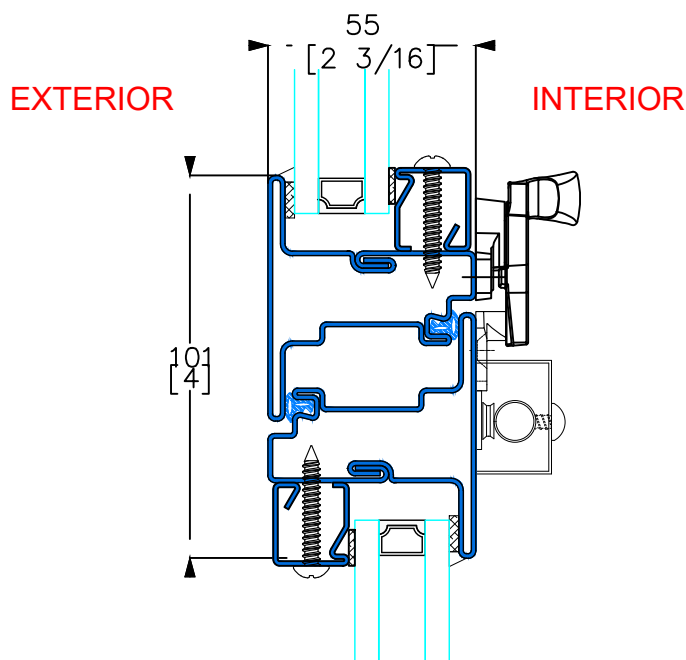
P TYPICAL STACKING HEAD
