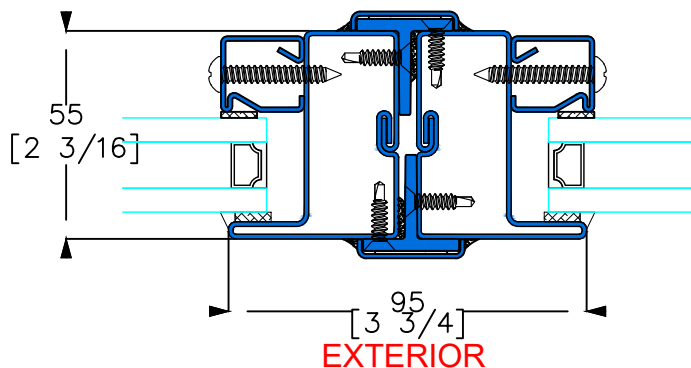
T TYPICAL FIXED JOINING MULLION
