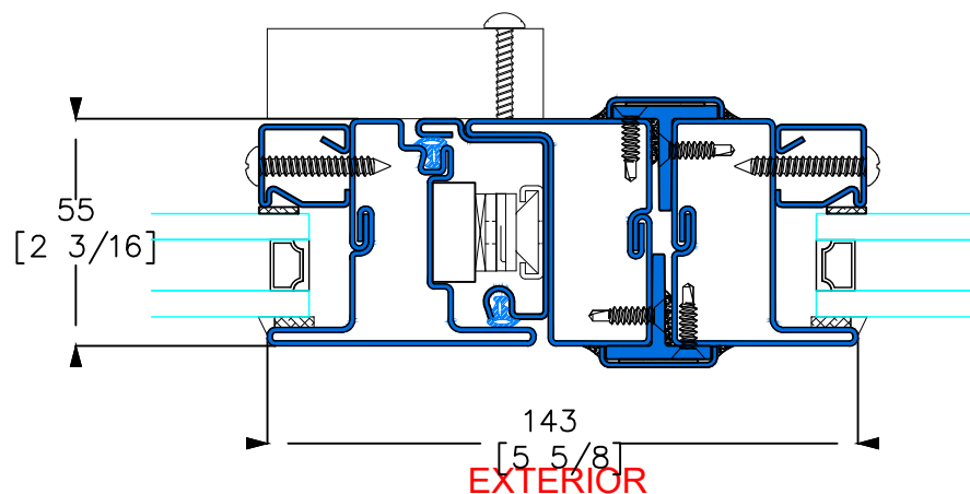
X TYPICAL JOINING MULLION
