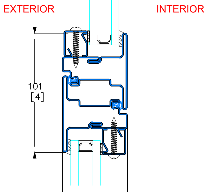
R TYPICAL STACKING MULLION
