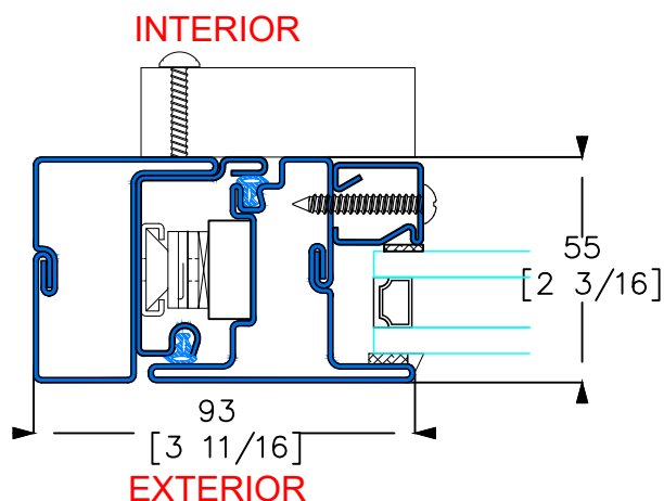
M&N TYPICAL STACKING JAMB
