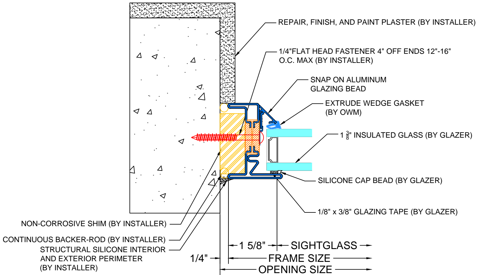
2 TYPICAL DETAIL DIRECT MOUNT
