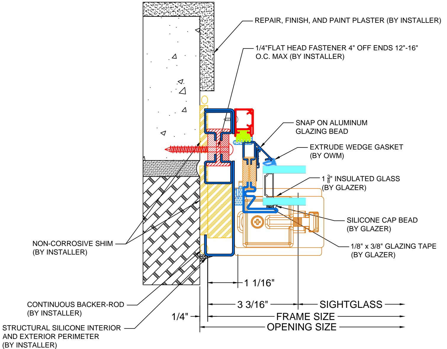
1 TYPICAL DETAIL DIRECT MOUNT
