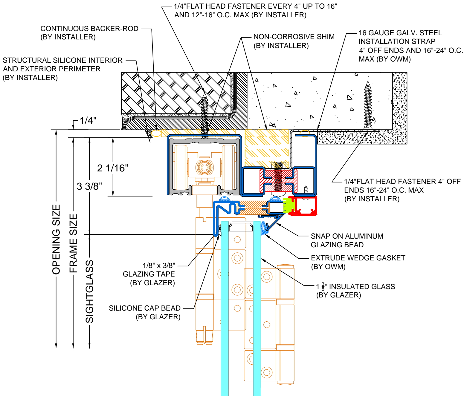
2 TYPICAL DETAIL DIRECT MOUNT
