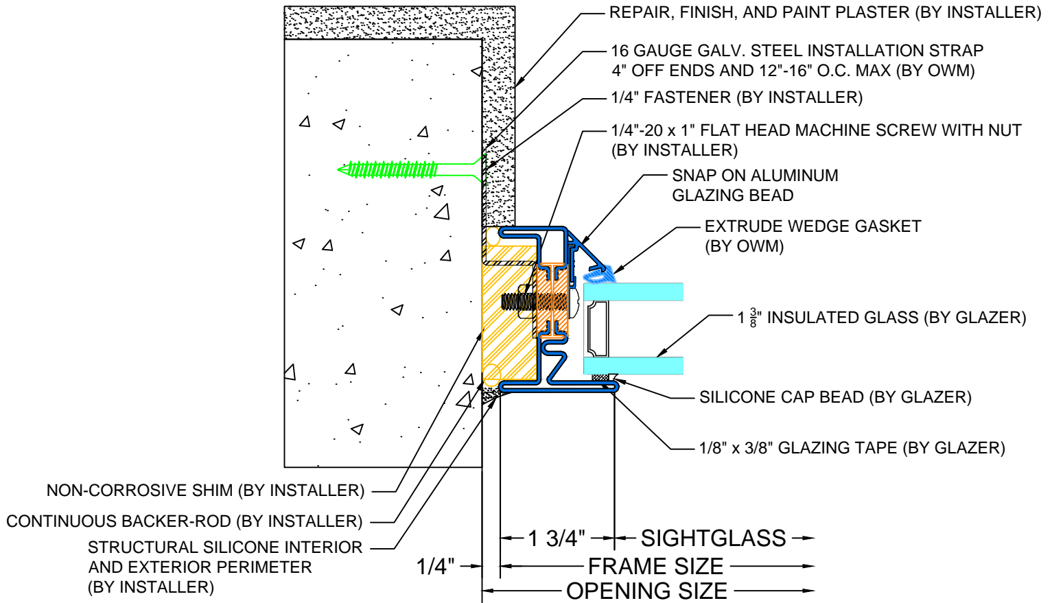
1 TYPICAL DETAIL INSTALLATION STRAP
