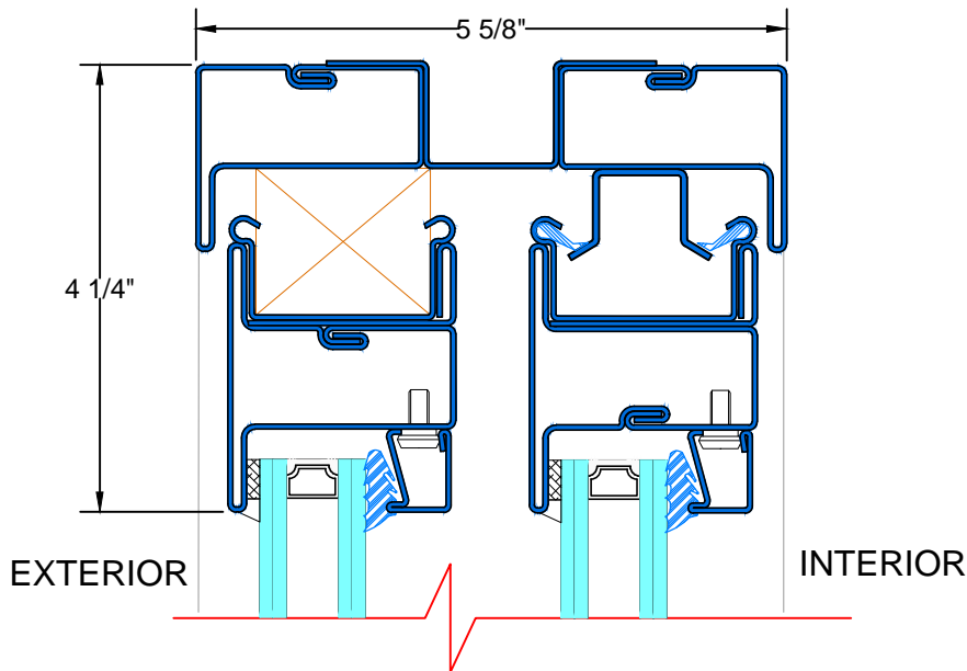
F TYPICAL HEAD INTERIOR ONE OPERABLE
