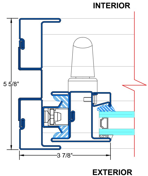
L TYPICAL JAMB OPERABLE
