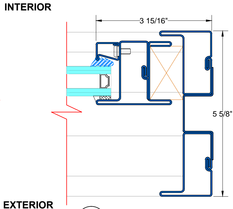
N TYPICAL JAMB FIXED
