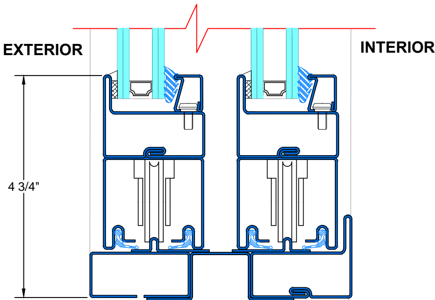
J TYPICAL SILL BOTH OPERABLE
