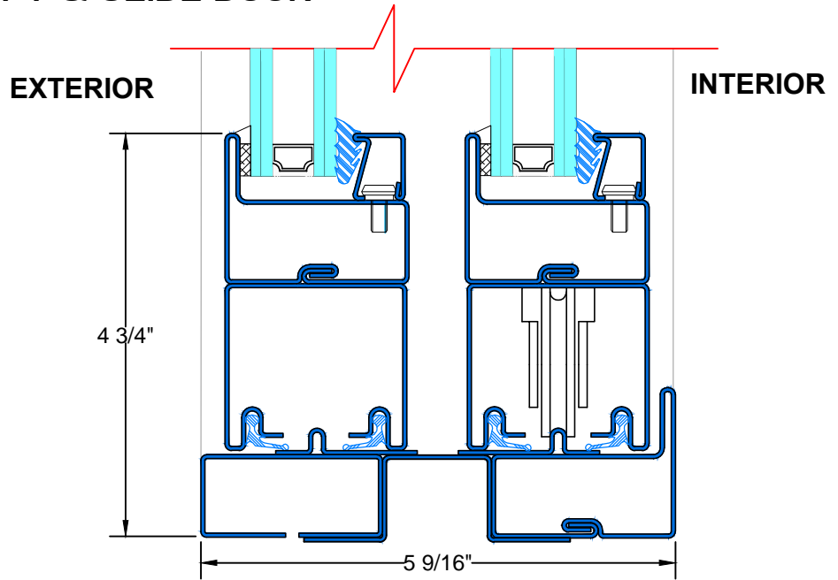
G TYPICAL SILL INTERIOR ONE OPERABLE
