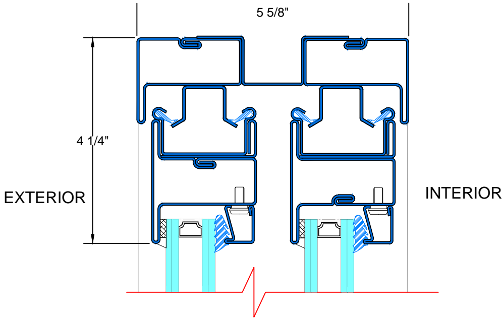
H TYPICAL HEAD BOTH OPERABLE
