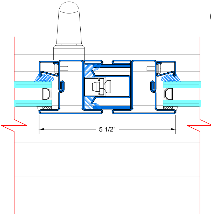
M TYPICAL FRENCH MEETING RAIL ONE OPERABLE
