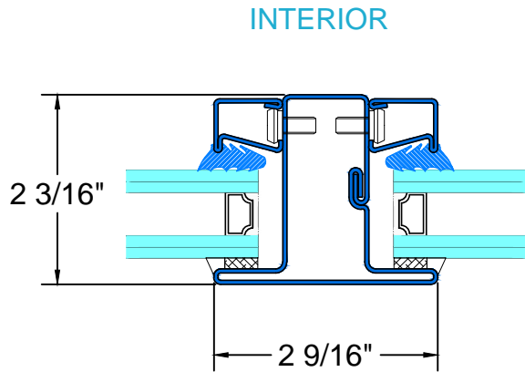
H TYPICAL VERTICAL MUNTIN
