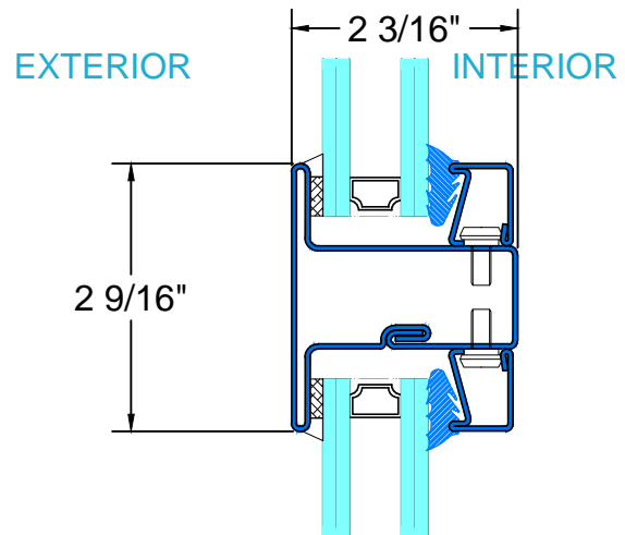
J TYPICAL HORIZONTAL MUNTIN
