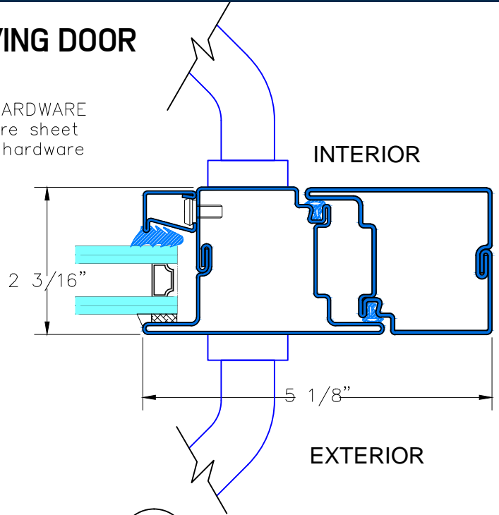
C TYPICAL LOCKING JAMB
