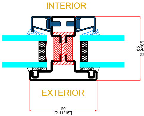
E TYPICAL VERTICAL MUNTIN
