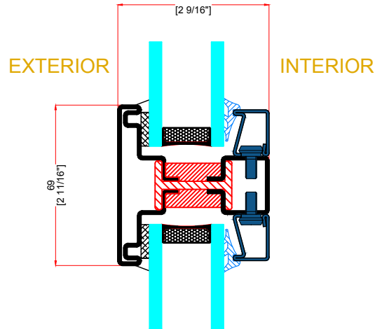
F TYPICAL HORIZONTAL MUNTIN
