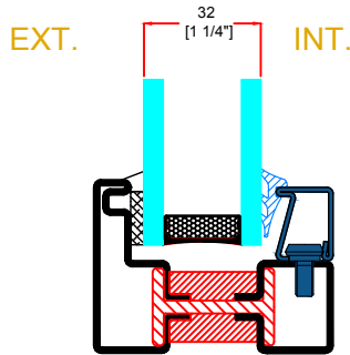
GB-2007 GLAZING BEAD
