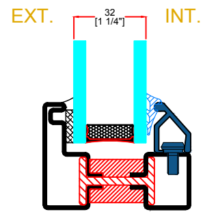
GB-1015 GLAZING BEAD
