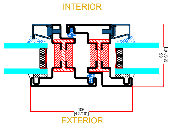
E — TYPICAL FRENCH MEETING RAIL
