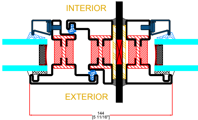
S TYPICAL JOINING MULLION
