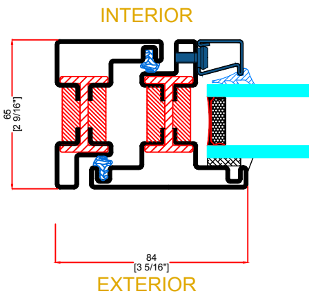
A&B — TYPICAL HINGED JAMB
