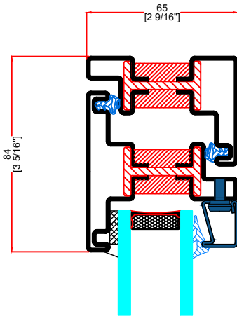
F TYPICAL HEAD
