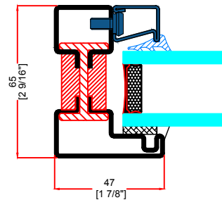
M&N TYPICAL FIXED JAMB
