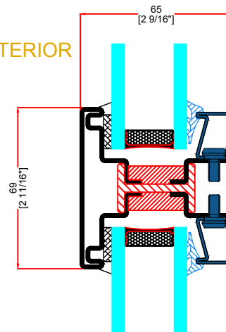
J TYPICAL HORIZONTAL MUNTIN
