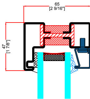
K&L TYPICAL FIXED HEAD & SILL
