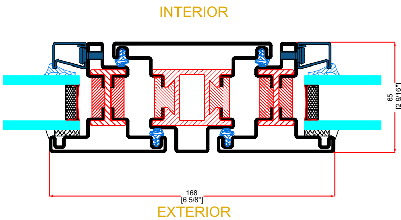
D — TYPICAL MEETING RAIL
