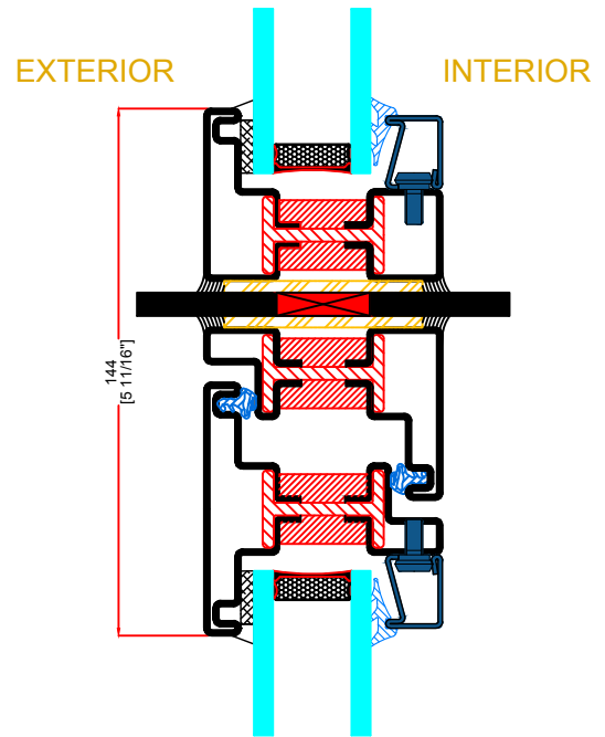
T TYPICAL STACKING TRANSOM
