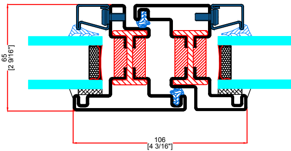
R TYPICAL JOINING SIDELITE
