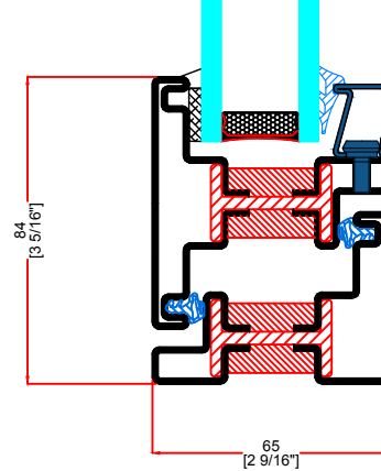
G TYPICAL SILL
