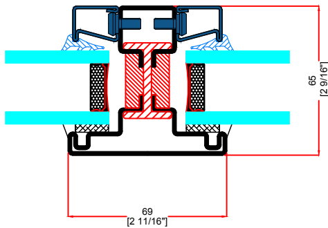
H TYPICAL VERTICAL MUNTIN
