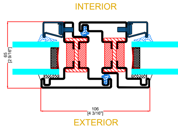
2 TYPICAL JAMB EXTERIOR FLANGE
