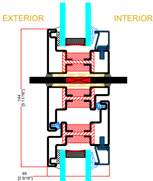
P TYPICAL STACKING MULLION
