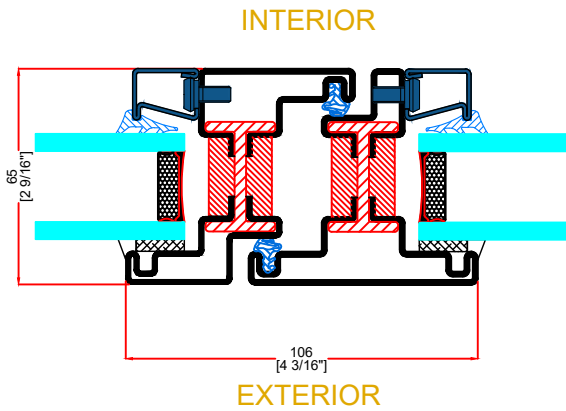
M TYPICAL JAMB WITH SIDELITE
