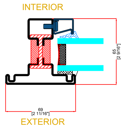
4 TYPICAL FIXED EXTERIOR FLANGE
