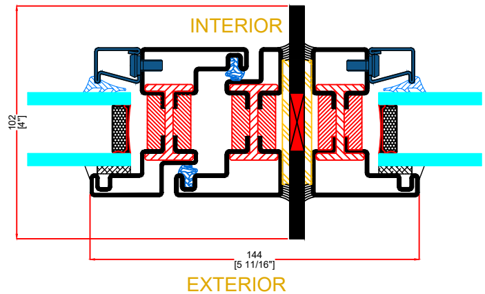
R TYPICAL JOINING MULLION
