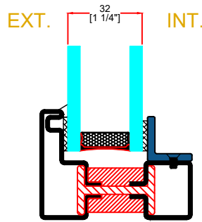
GB18-.75 GLAZING BEAD
