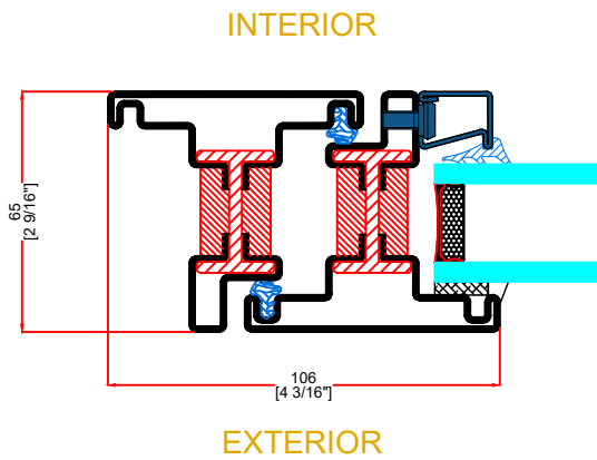
1 TYPICAL JAMB INTERIOR FLANGE
