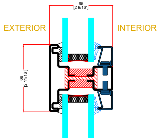
G TYPICAL HORIZONTAL MUNTIN
