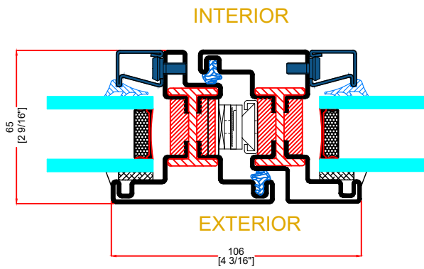
M TYPICAL JAMB WITH SIDELITE
