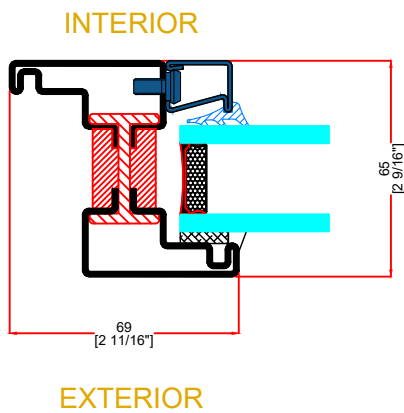
3 TYPICAL FIXED INTERIOR FLANGE
