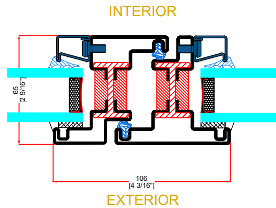
2 TYPICAL JAMB EXTERIOR FLANGE
