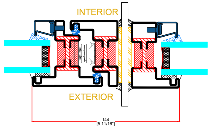
R TYPICAL JOINING MULLION
