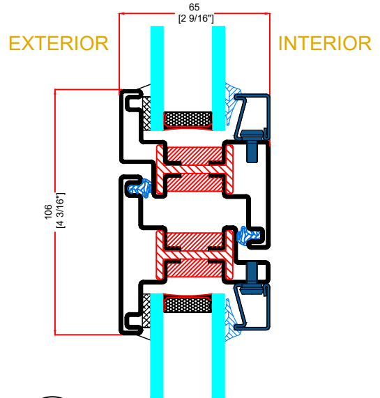
N TYPICAL HEAD WITH TRANSOM
