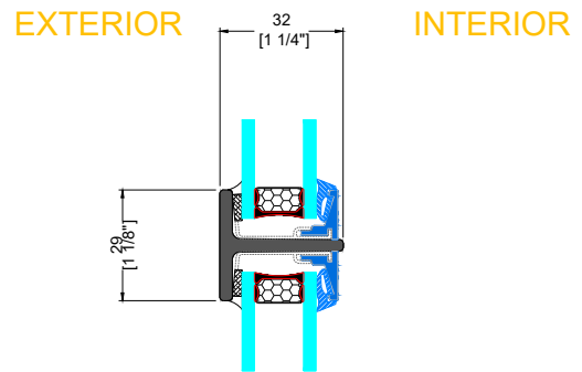
F TYPICAL HORIZONTAL MUNTIN
