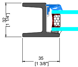
A TYPICAL LEFT JAMB
