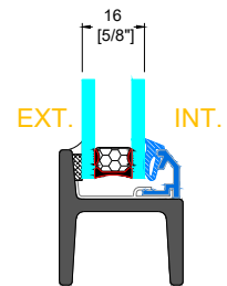
GB-12 GLAZING BEAD
