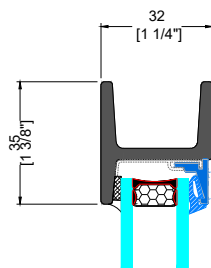
C TYPICAL HEAD
