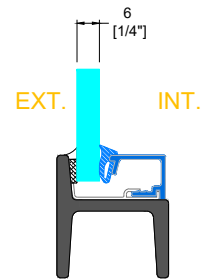
GB-06 GLAZING BEAD
