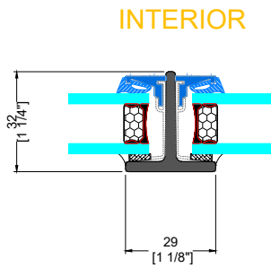
E TYPICAL VERTICAL MUNTIN
