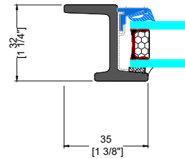
2 TYPICAL FIXED INTERIOR FLANGE
