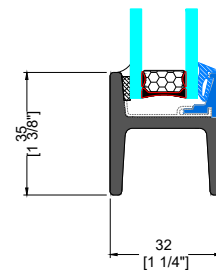
D TYPICAL SILL
