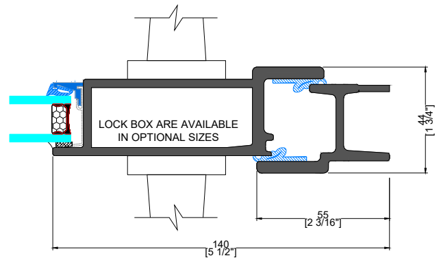
E TYPICAL SINGLE LOCKBOX
