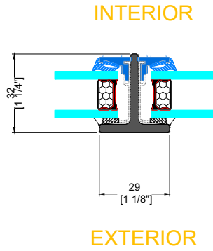
J TYPICAL VERTICAL MUNTIN
