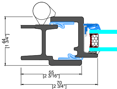
A&B TYPICAL HINGED JAMB
