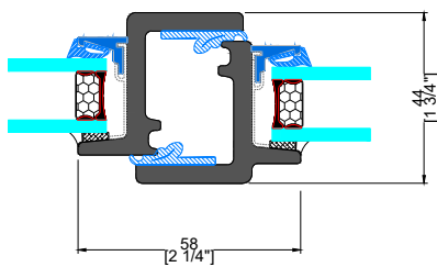
D TYPICAL FRENCH MEETING RAIL
