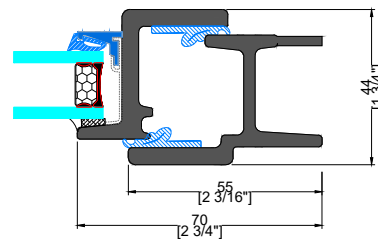
C TYPICAL LOCKING JAMB
