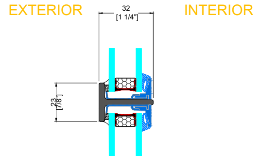
K SMALL HORIZONTAL MUNTIN
