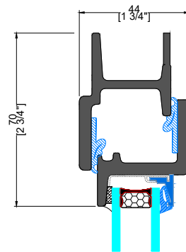
F TYPICAL HEAD
