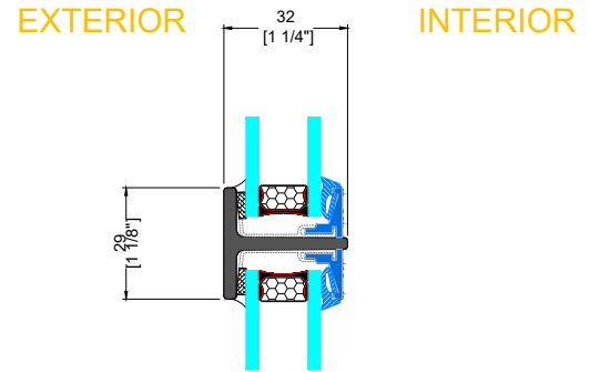
K TYPICAL HORIZONTAL MUNTIN
