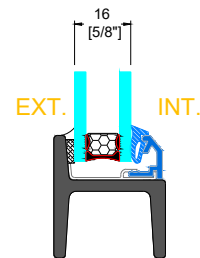
GB-12 GLAZING BEAD
