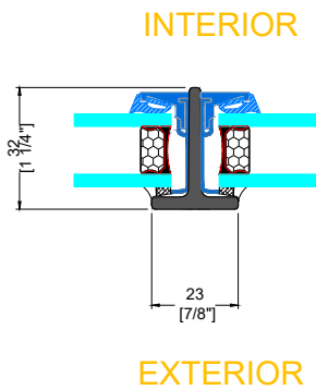
J SMALL VERTICAL MUNTIN
