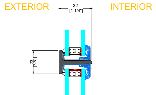
K SMALL HORIZONTAL MUNTIN
