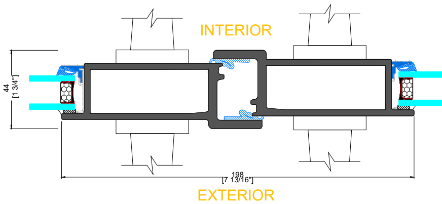
F TYPICAL FRENCH LOCKBOX
