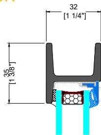
L&M TYPICAL FIXED HEAD & SILL
