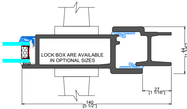
D TYPICAL SINGLE LOCKBOX
