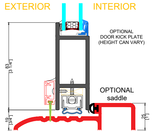
H TYPICAL KICKPLATE
