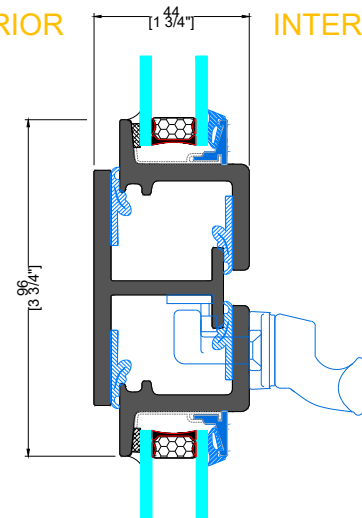
E TYPICAL STACKING MULLION
