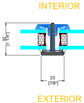
F SMALL VERTICAL MUNTIN
