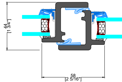
N TYPICAL JAMB W/ SIDELITE
