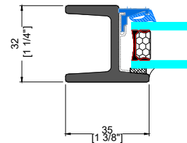
K&L TYPICAL FIXED JAMB
