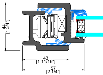
A&B TYPICAL HINGED JAMB
