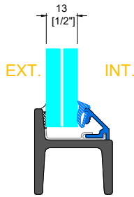
GB-04 GLAZING BEAD
