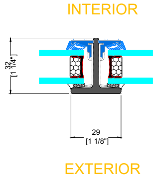
F TYPICAL VERTICAL MUNTIN
