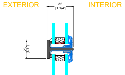
G SMALL HORIZONTAL MUNTIN
