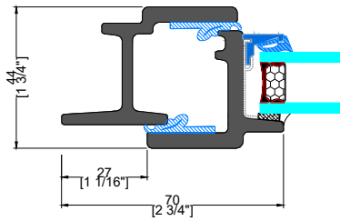
1 TYPICAL JAMB EXTERIOR FLANGE
