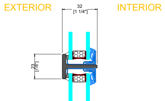
G SMALL HORIZONTAL MUNTIN
