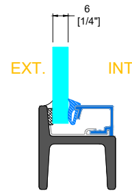
GB-06 GLAZING BEAD
