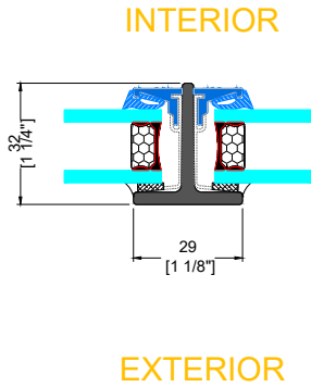
F TYPICAL VERTICAL MUNTIN
