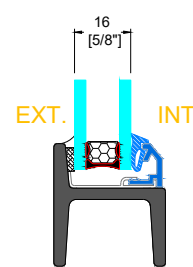
GB-12 GLAZING BEAD
