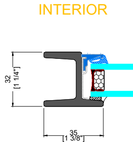
K&L TYPICAL FIXED JAMB
