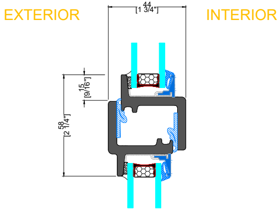
M TYPICAL HEAD W/ TRANSOM
