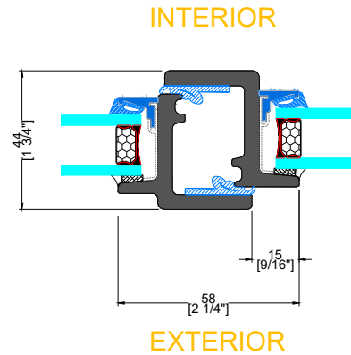
N TYPICAL JAMB W/ SIDELITE
