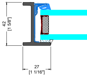
A TYPICAL LEFT JAMB
