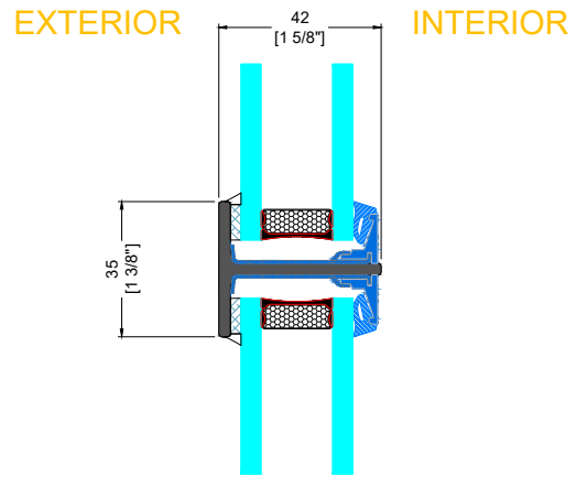
F TYPICAL HORIZONTAL MUNTIN
