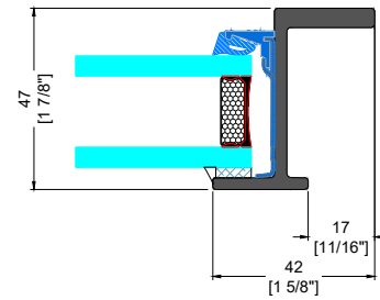
2 TYPICAL INTERIOR FLANGE
