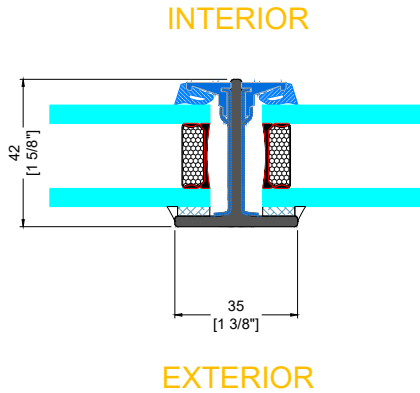
E TYPICAL VERTICAL MUNTIN
