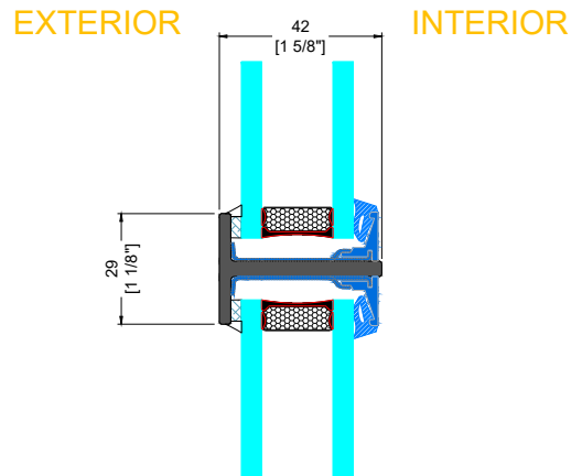
F SMALL HORIZONTAL MUNTIN
