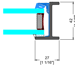
B TYPICAL RIGHT JAMB
