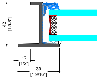
1 TYPICAL EXTERIOR FLANGE
