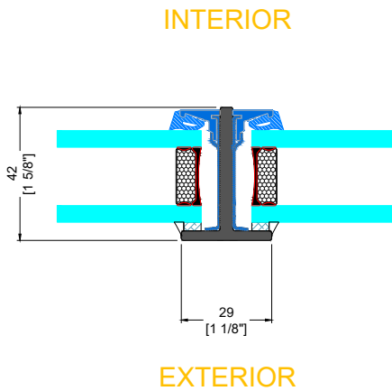
E SMALL VERTICAL MUNTIN
