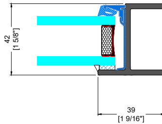
3 TYPICAL LONG LEG FRAME
