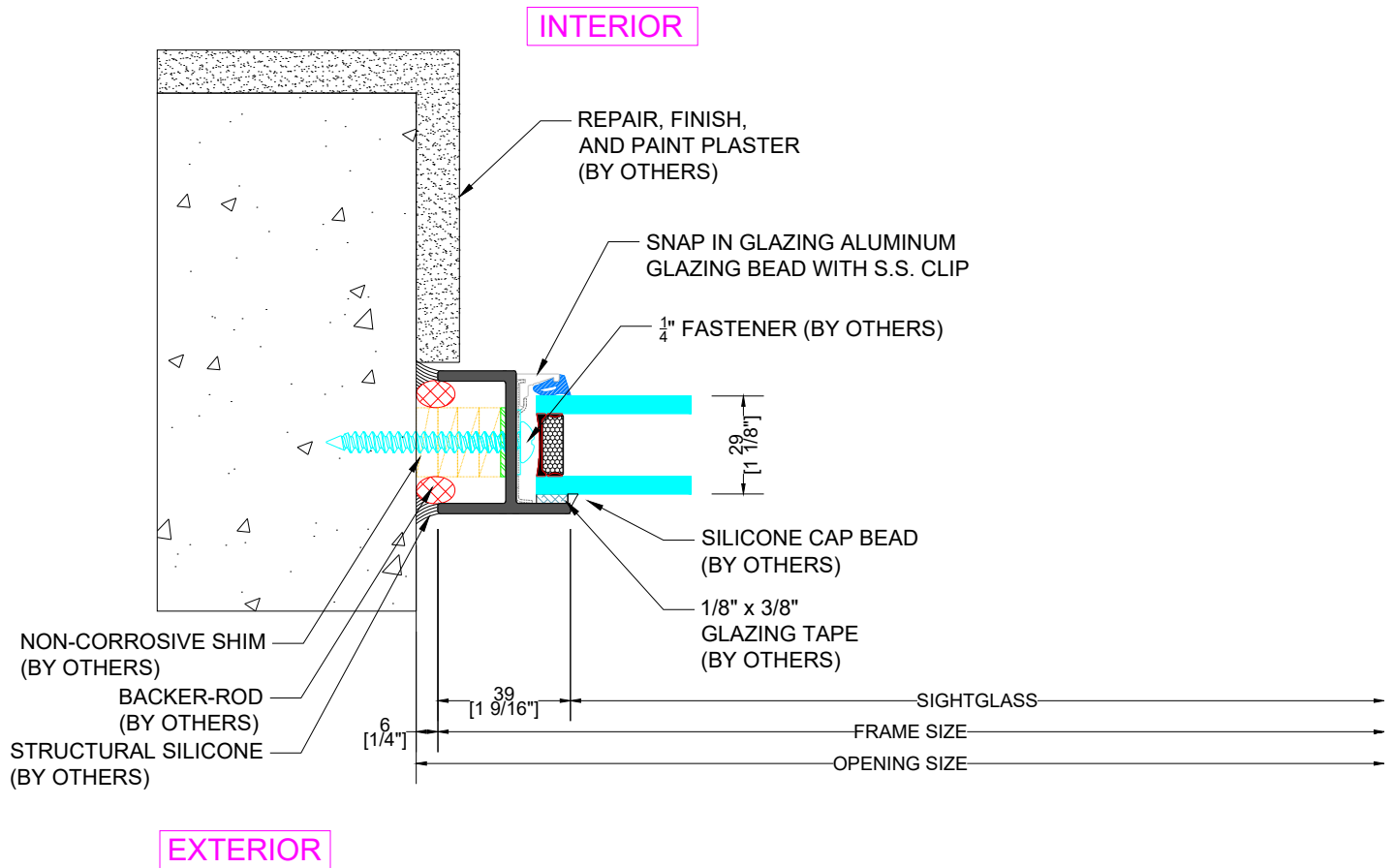
1 TYPICAL DETAIL DIRECT FIX
