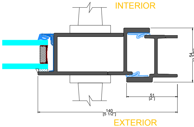
E TYPICAL LOCKBOX SINGLE DOOR
