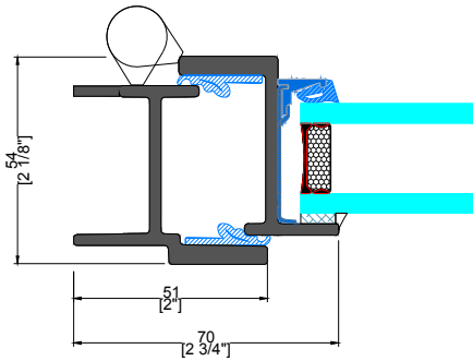
A&B TYPICAL HINGED JAMB
