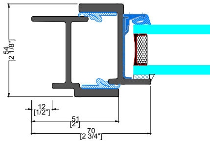
1 TYPICAL INTERIOR FLANGE
