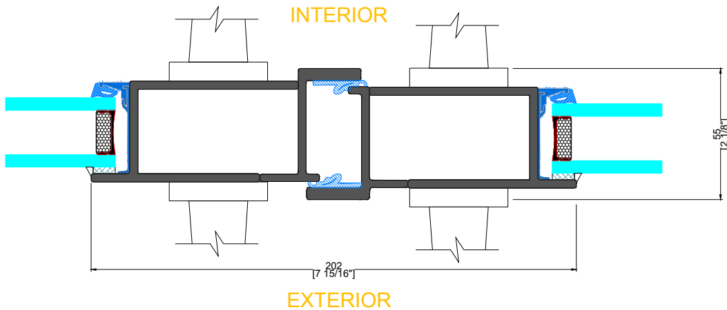
F TYPICAL LOCKBOX FRENCH DOOR
