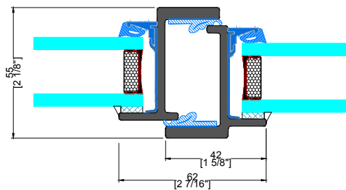
D TYPICAL FRENCH MEETING RAIL
