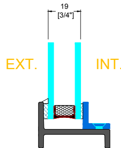
1/2" x 3/4" STEEL GLAZING BEAD
