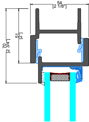
G TYPICAL HEAD
