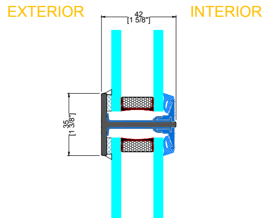
K TYPICAL HORIZONTAL MUNTIN
