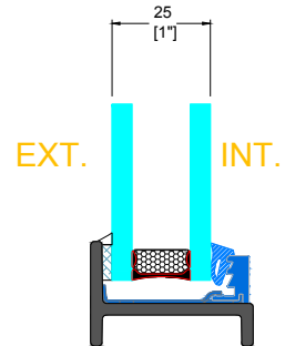
GB-13X ALUMINUM GLAZING BEAD
