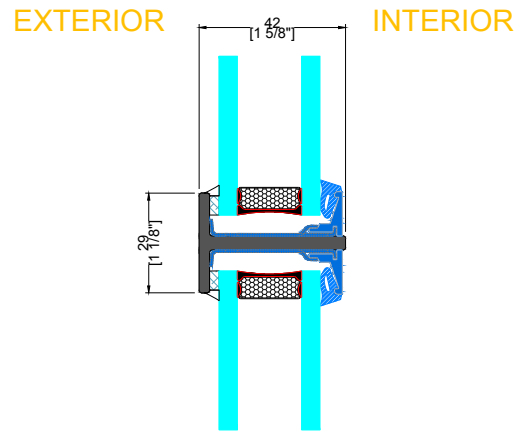
K SMALL HORIZONTAL MUNTIN
