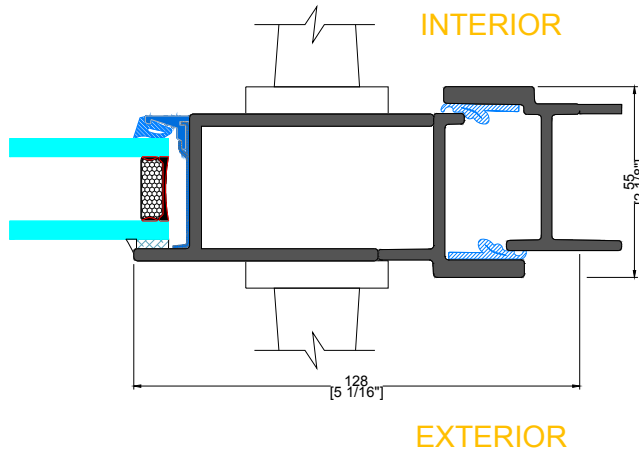
E TYPICAL LOCKBOX SINGLE DOOR
