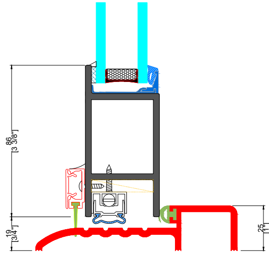
H TYPICAL KICKPLATE
