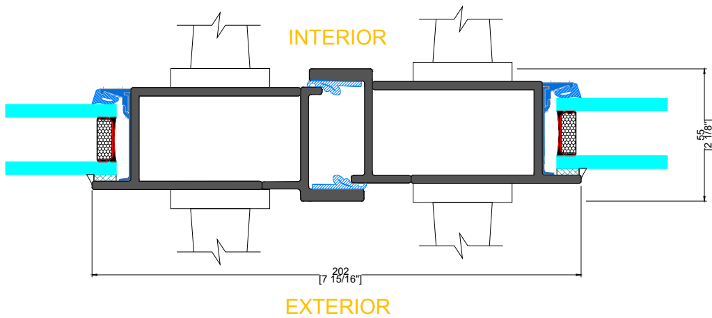
F TYPICAL LOCKBOX FRENCH DOOR
