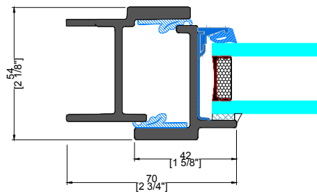
3 TYPICAL LONG LEG
