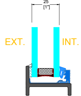
GB-13X ALUMINUM GLAZING BEAD
