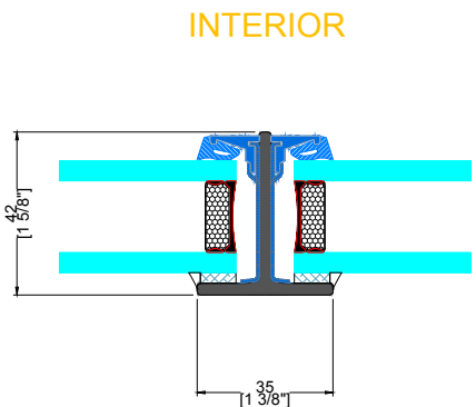
J TYPICAL VERTICAL MUNTIN
