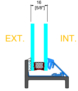
GB-15X GLAZING BEAD
