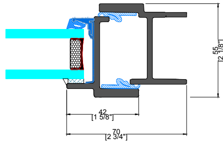
C TYPICAL LOCKING JAMB
