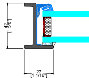
N&P TYPICAL FIXED JAMB
