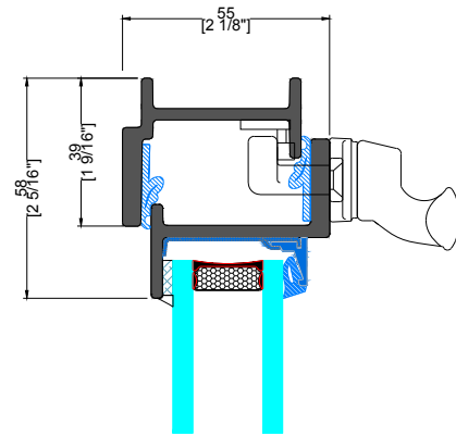
C TYPICAL LOCKING HEAD
