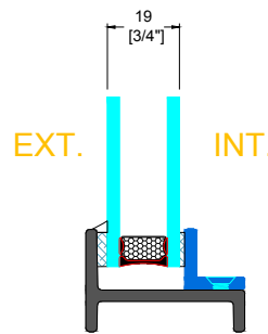
1/2" x 3/4" STEEL GLAZING BEAD
