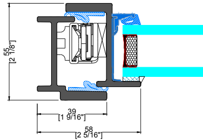
A&B TYPICAL HINGED JAMB
