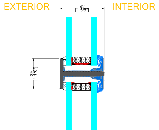
G SMALL HORIZONTAL MUNTIN
