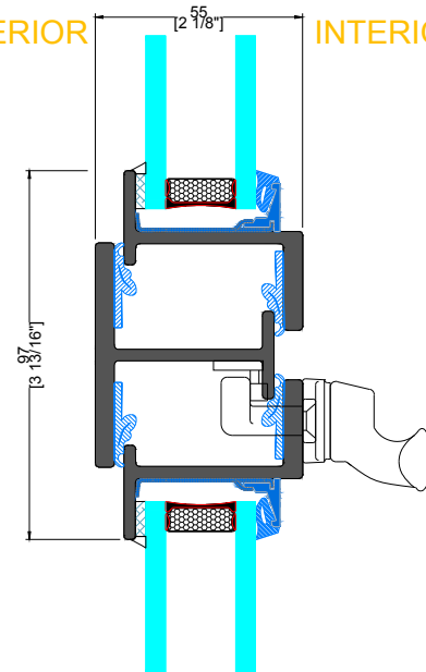
E TYPICAL STACKING JOINT
