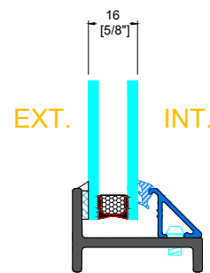
GB-35 GLAZING BEAD
