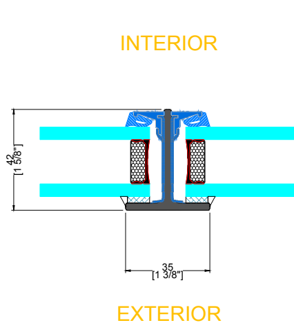
F TYPICAL VERTICAL MUNTIN
