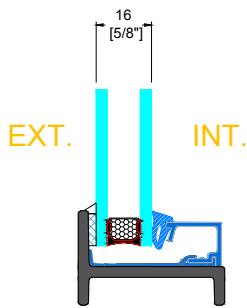
GB-06X GLAZING BEAD
