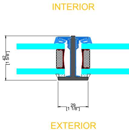
F SMALL VERTICAL MUNTIN
