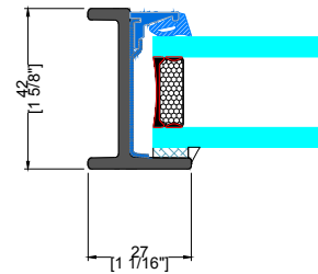
K&L TYPICAL FIXED JAMB
