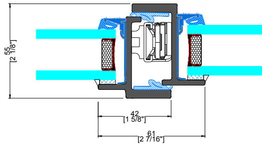
N TYPICAL JAMB W/ SIDELITE
