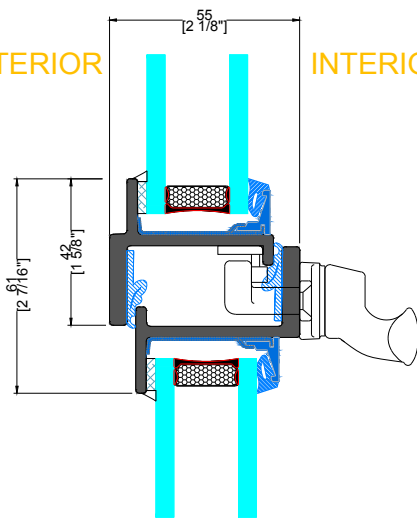
M TYPICAL HEAD W/ TRANSOM
