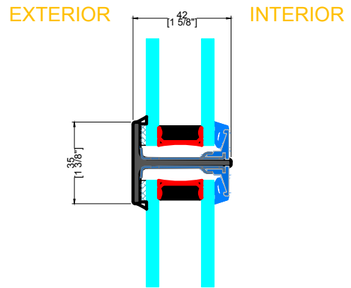
G TYPICAL HORIZONTAL MUNTIN
