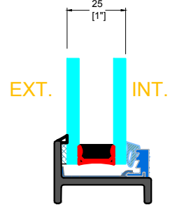
GB-13X GLAZING BEAD
