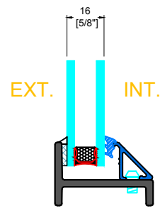
GB-35 GLAZING BEAD
