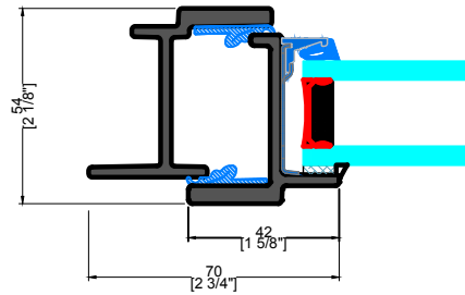
2 TYPICAL EXTERIOR FLANGE
