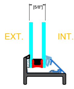
GB-15X GLAZING BEAD
