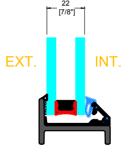
GB-04X GLAZING BEAD
