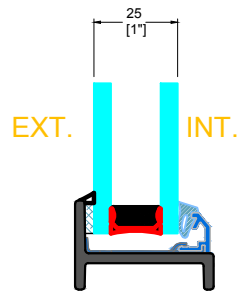
GB-12X GLAZING BEAD
