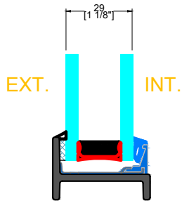
GB-05X GLAZING BEAD
