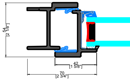
3 TYPICAL LONG LEG
