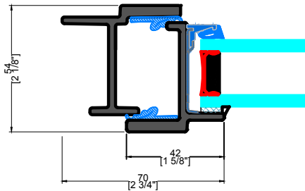
1 TYPICAL INTERIOR FLANGE
