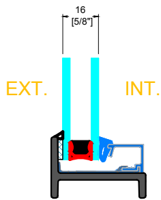
GB-06X GLAZING BEAD
