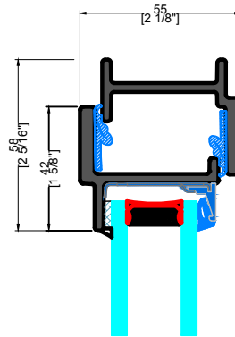
C TYPICAL HEAD
