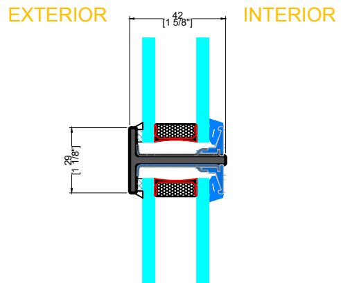
G TYPICAL HORIZONTAL MUNTIN
