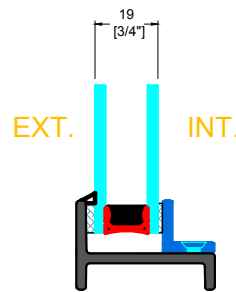
1/2" x 3/4" STEEL GLAZING BEAD
