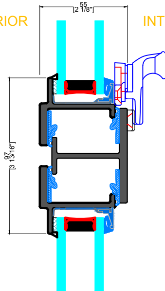
E TYPICAL STACKING JOINT
