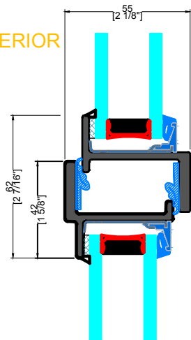
M TYPICAL HEAD W/ TRANSOM
