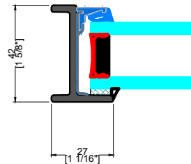
K&L TYPICAL FIXED JAMB
