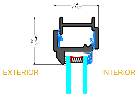
D TYPICAL HEAD
