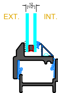
GB-35 GLAZING BEAD
