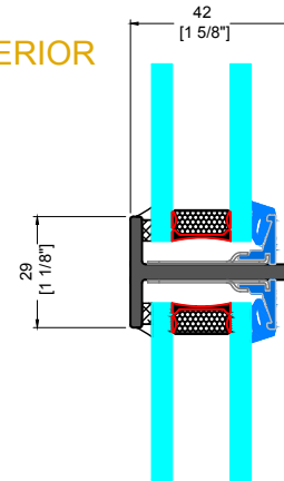
F TYPICAL HORIZONTAL MUNTIN
