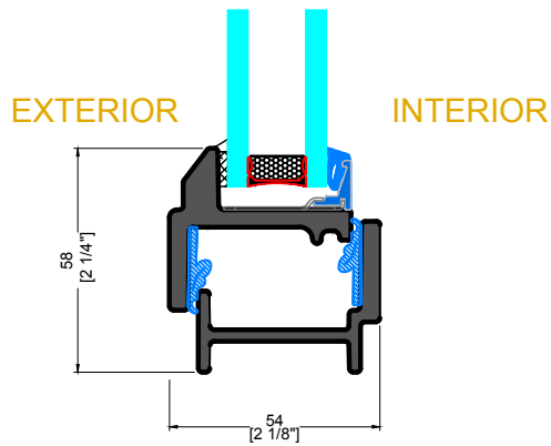
C TYPICAL SILL
