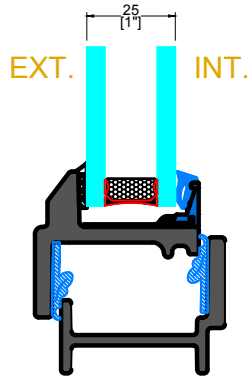
GB-05X GLAZING BEAD
