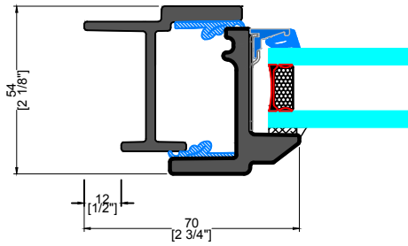
1 TYPICAL JAMB INTERIOR FLANGE
