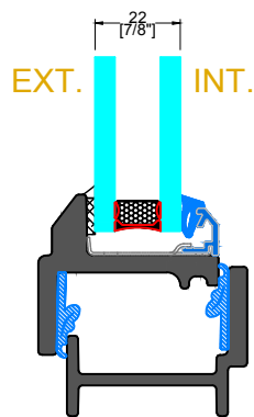
GB-12X GLAZING BEAD
