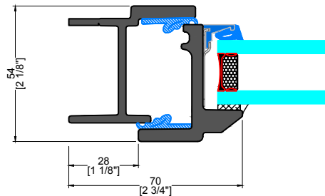
3 TYPICAL JAMB LONG LEG
