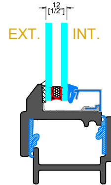
GB-06X GLAZING BEAD
