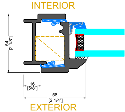
K&L TYPICAL FIXED JAMB
