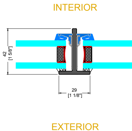
F TYPICAL SMALL VERTICAL MUNTIN
