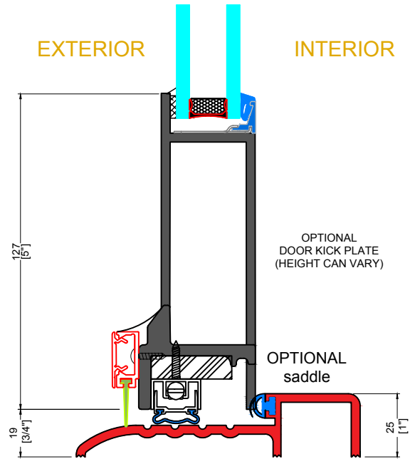
E TYPICAL KICKPLATE
