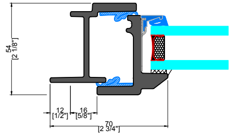
2 TYPICAL JAMB EXTERIOR FLANGE
