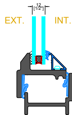
GB-35 GLAZING BEAD
