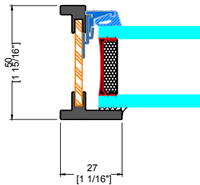
A TYPICAL LEFT JAMB
