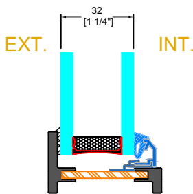
GB-12 GLAZING BEAD
