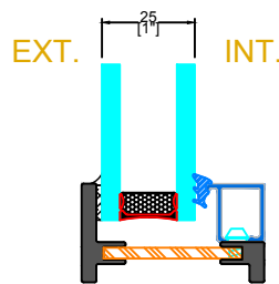
GB-31 GLAZING BEAD
