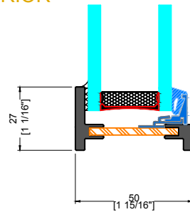
D TYPICAL SILL
