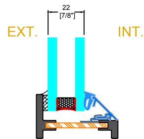
GB-15 GLAZING BEAD
