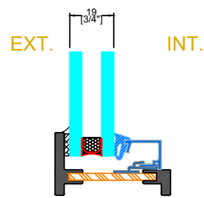
GB-06 GLAZING BEAD
