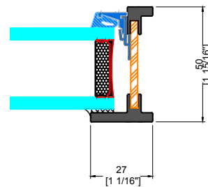
B TYPICAL RIGHT JAMB
