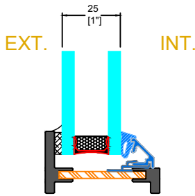
GB-04 GLAZING BEAD
