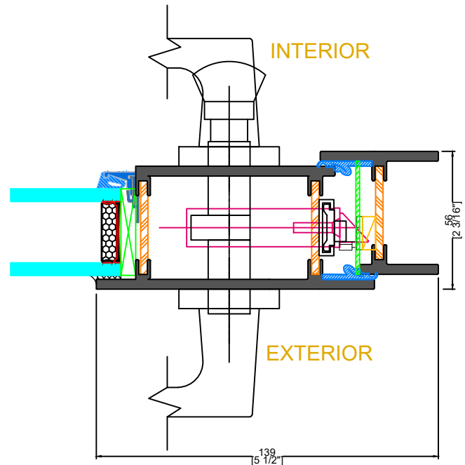
E TYPICAL SINGLE LOCKBOX
