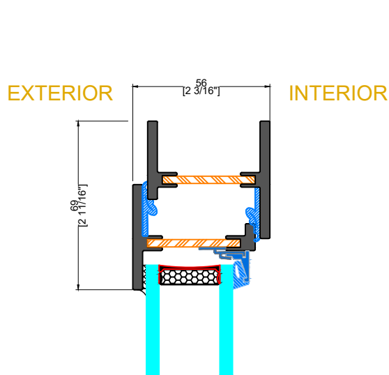
G TYPICAL HEAD
