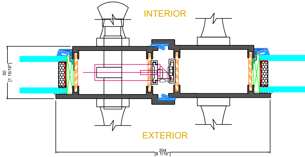
F TYPICAL FRENCH LOCKBOX
