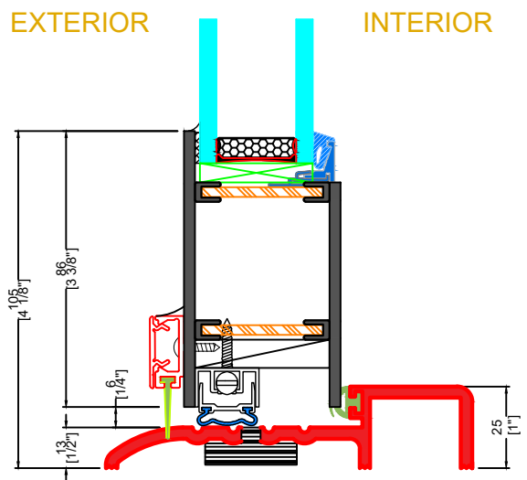
H TYPICAL KICKPLATE
