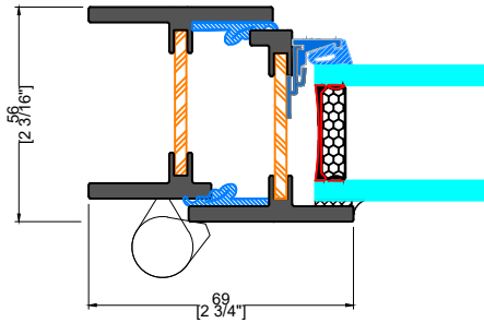
A&B TYPICAL HINGED JAMB
