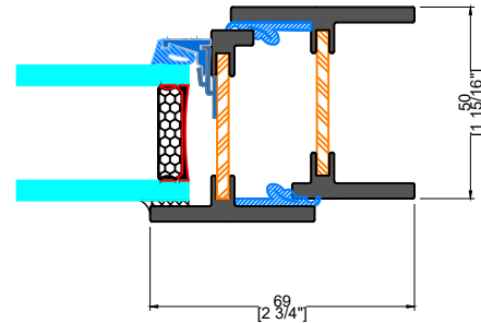
C TYPICAL LOCKING JAMB
