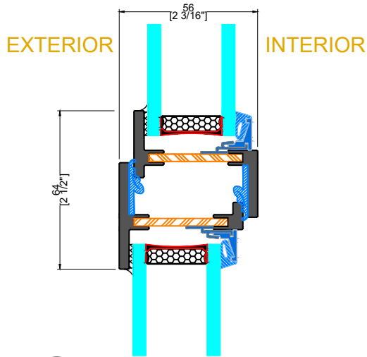
R TYPICAL HEAD W/ TRANSOM
