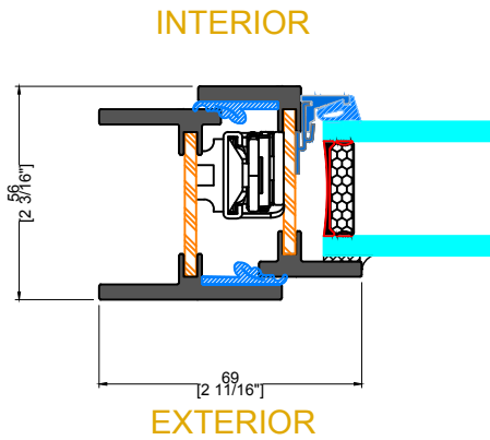
1 TYPICAL JAMB EXTENDED FLANGE
