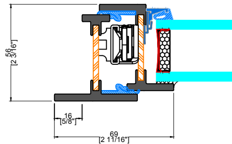
2 TYPICAL JAMB EXTERIOR FLANGE
