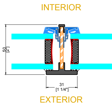
F TYPICAL VERTICAL MUNTIN
