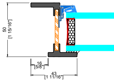
3 TYPICAL FIXED JAMB INTERIOR FLANGE
