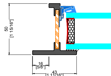
4 TYPICAL FIXED JAMB EXTERIOR FLANGE
