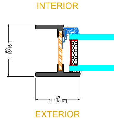
2 TYPICAL FIXED JAMB EXTENDED FLANGE
