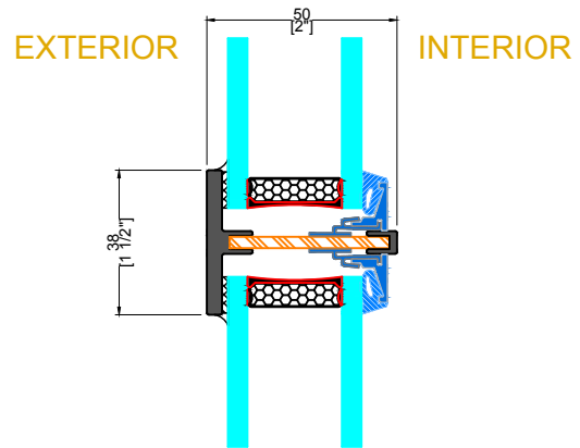
G TYPICAL HORIZONTAL MUNTIN
