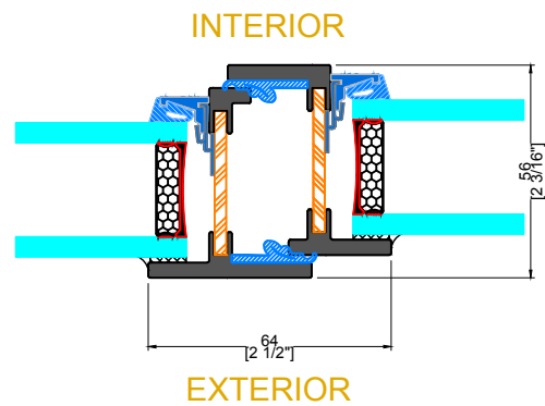
N TYPICAL JAMB W/ SIDELITE
