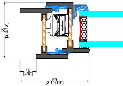
1 TYPICAL JAMB INTERIOR FLANGE
