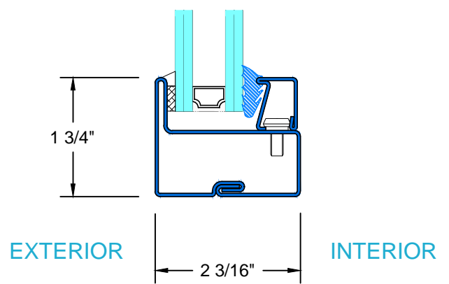
D TYPICAL SILL
