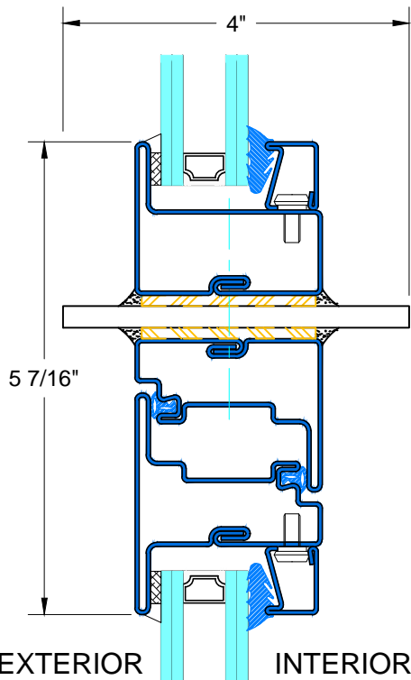
P TYPICAL STACKING MULLION
