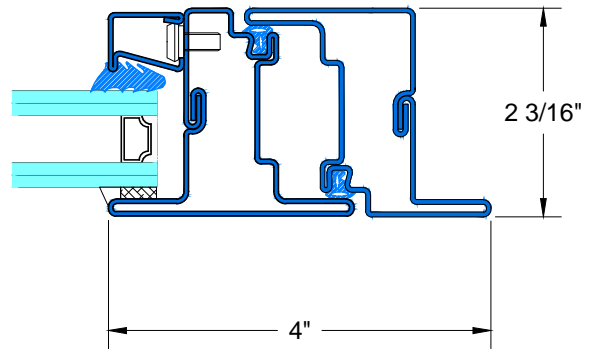
2 TYPICAL JAMB EXTERIOR FLANGE
