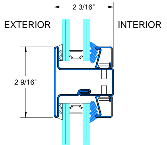
G TYPICAL HORIZONTAL MUNTIN
