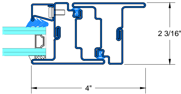
1 TYPICAL JAMB INTERIOR FLANGE
