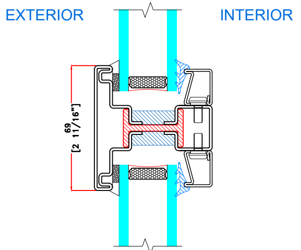
Q TYPICAL HORIZONTAL MUNTIN
