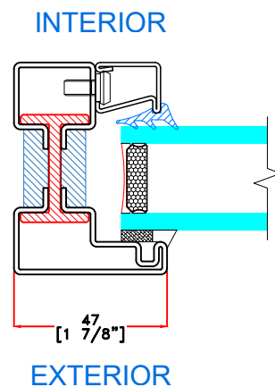
M&N TYPICAL FIXED JAMB
