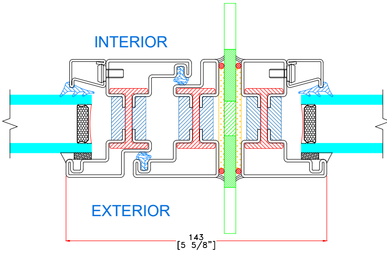
R TYPICAL JOINING MULLION
