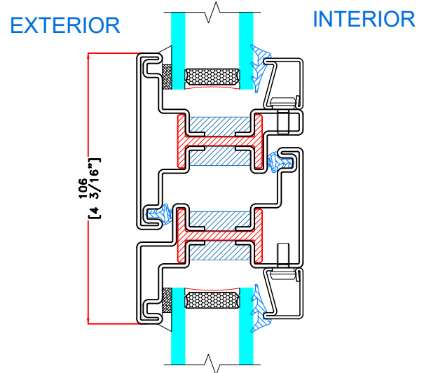
I TYPICAL FIXED/ OPERABLE MEETING RAIL
