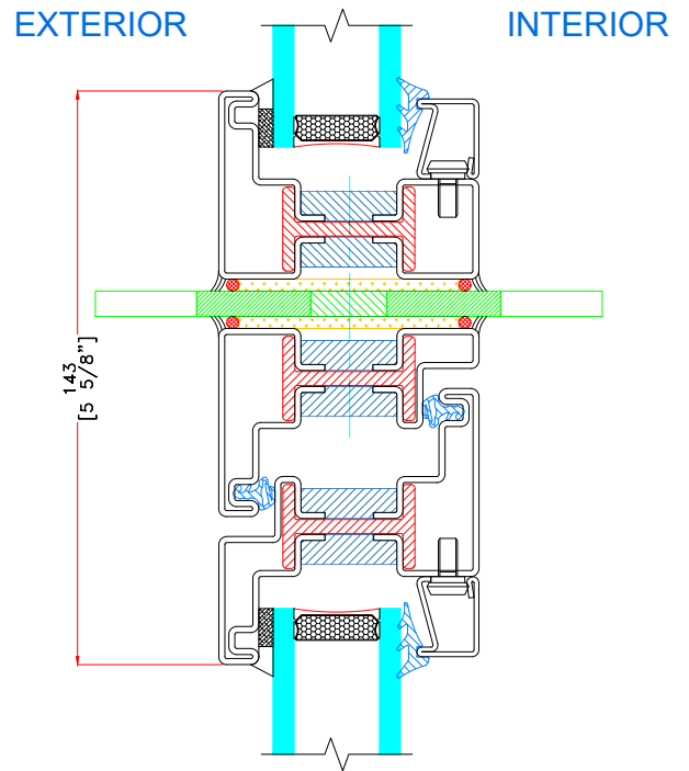
S TYPICAL STACKING MULLION
