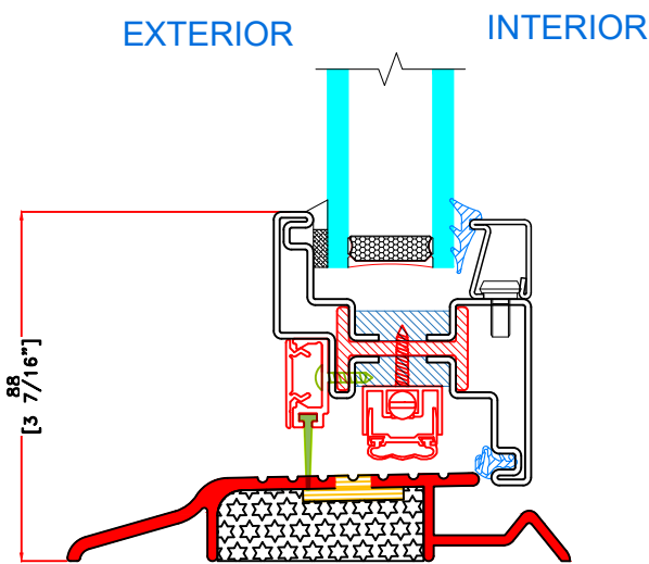
J TYPICAL KICKPALTE
