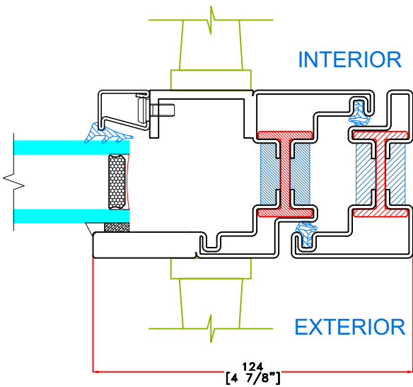
G TYPICAL SINGLE LOCKBOX
