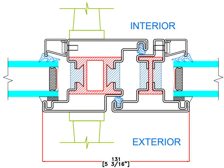
H TYPICAL FRENCH MEETING RAIL
