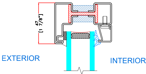
K&L TYPICAL FIXED HEAD & SILL
