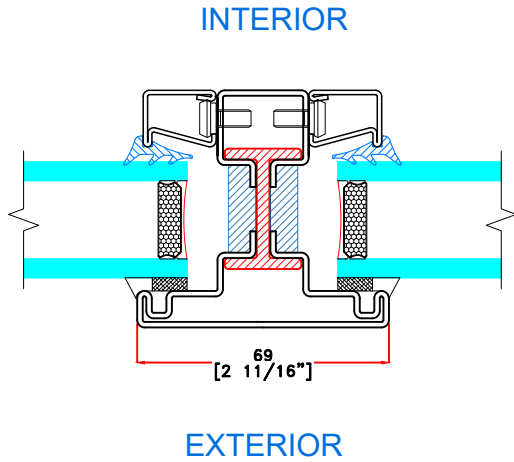
P TYPICAL VERTICAL MUNTIN
