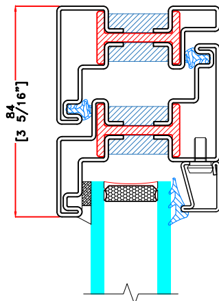
D TYPICAL HEAD
