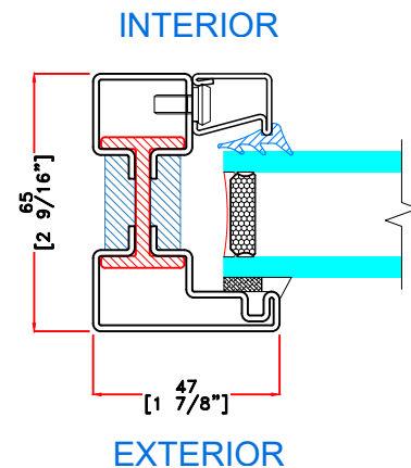
M&N TYPICAL FIXED JAMB
