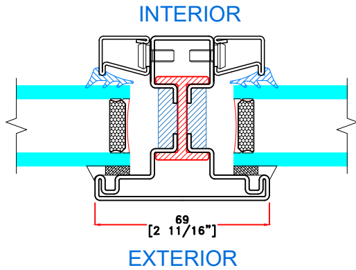
P TYPICAL VERTICAL MUNTIN
