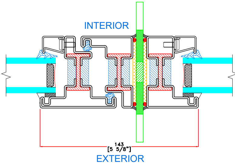
R TYPICAL JOINING MULLION
