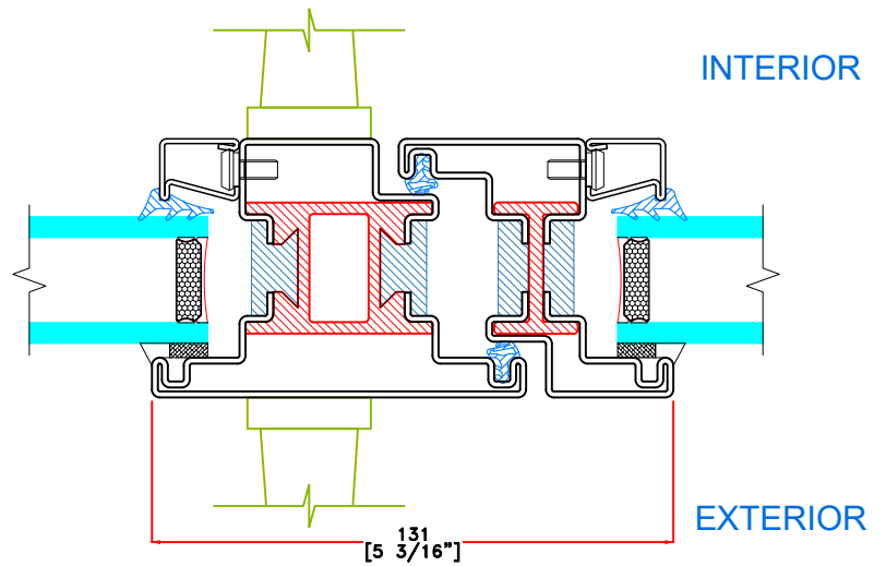
H OPTIONAL FRENCH MEETING RAIL
