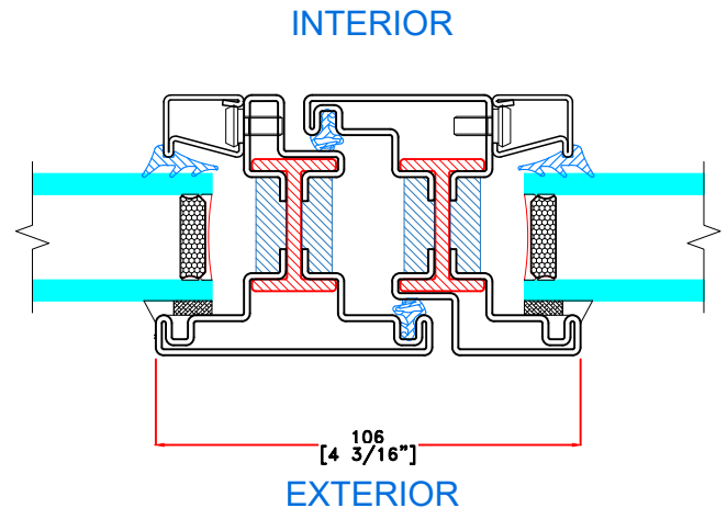
E TYPICAL FRENCH MEETING RAIL
