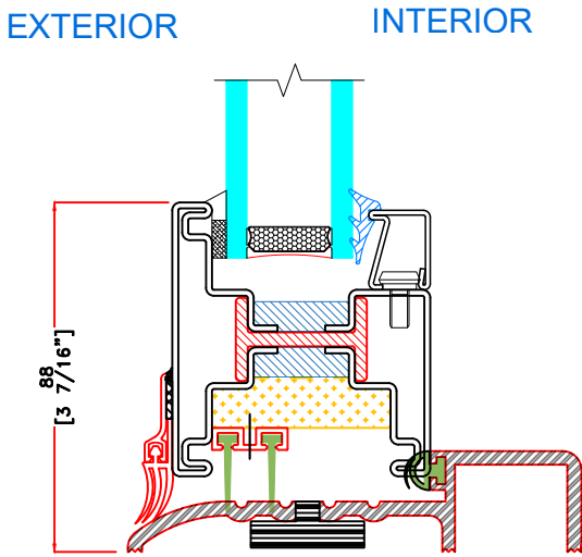
J TYPICAL KICKPALTE
