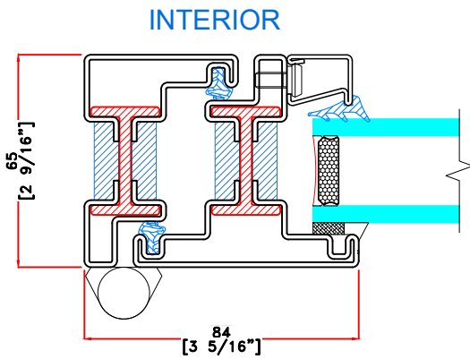
A&B TYPICAL HINGED JAMB
