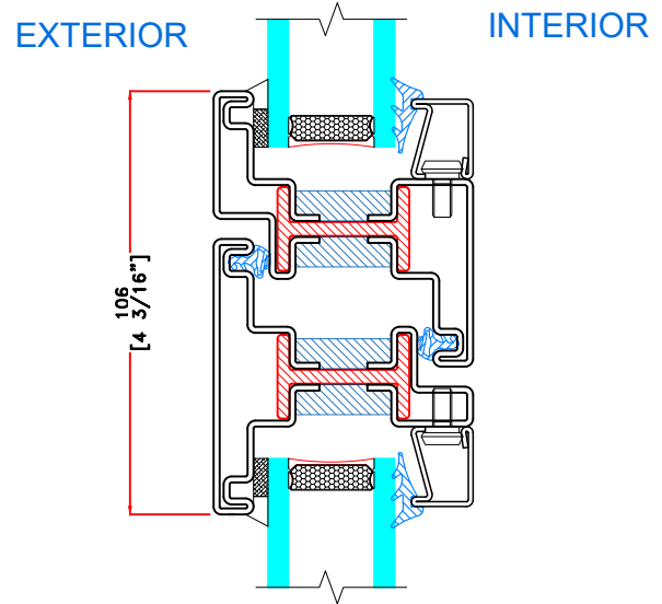
I TYPICAL FIXED/ OPERABLE MEETING RAIL
