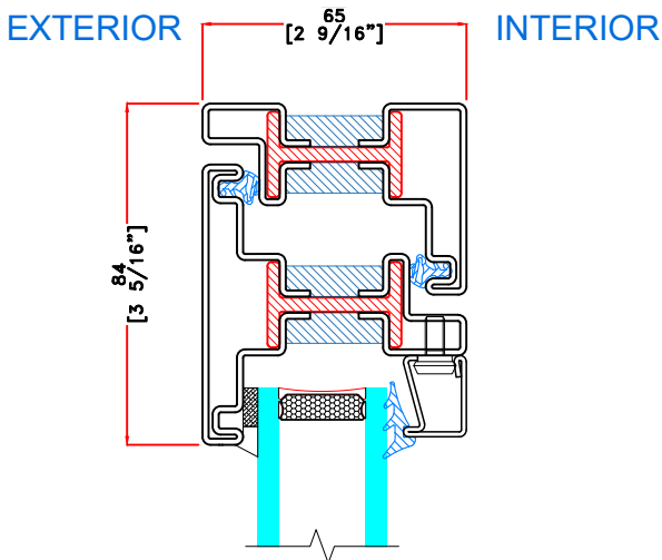
D TYPICAL HEAD
