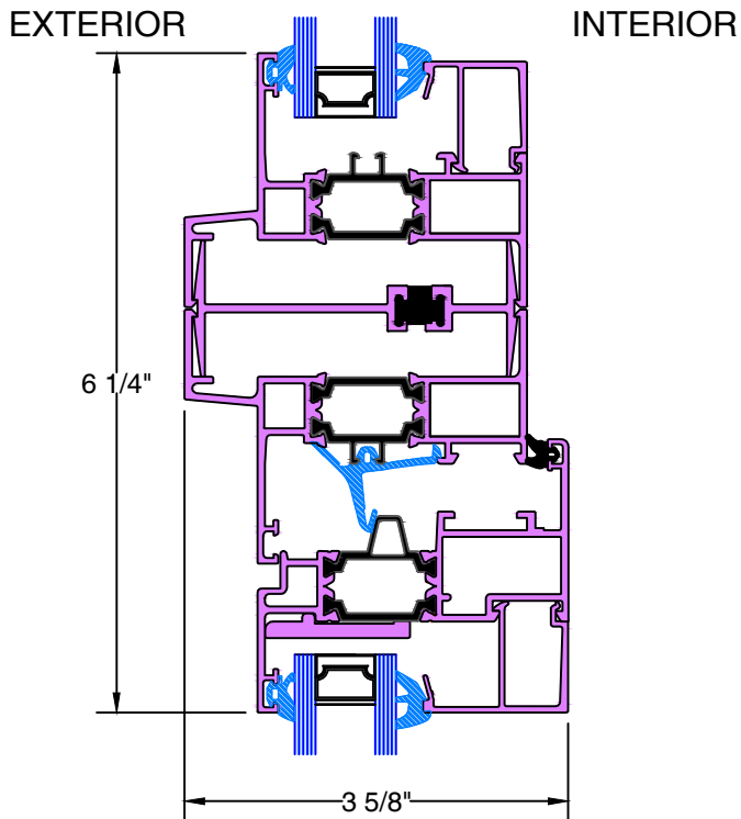
M TYPICAL STACKING MULLION
