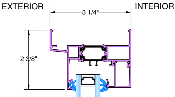
H&J TYPICAL FIXED HEAD & SILL
