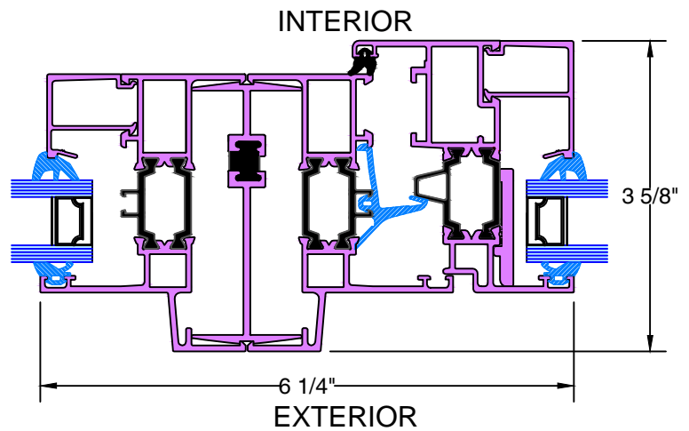
N TYPICAL JOINING MULLION
