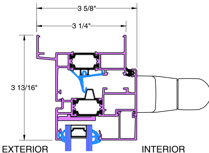
D TYPICAL HEAD
