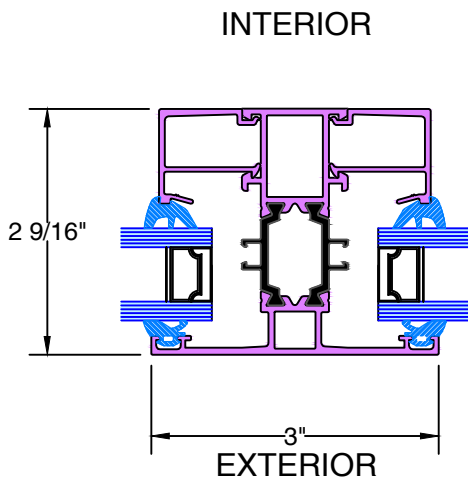
F TYPICAL VERTICAL MUNTIN
