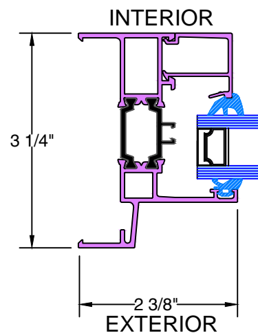
K&L TYPICAL FIXED JAMB
