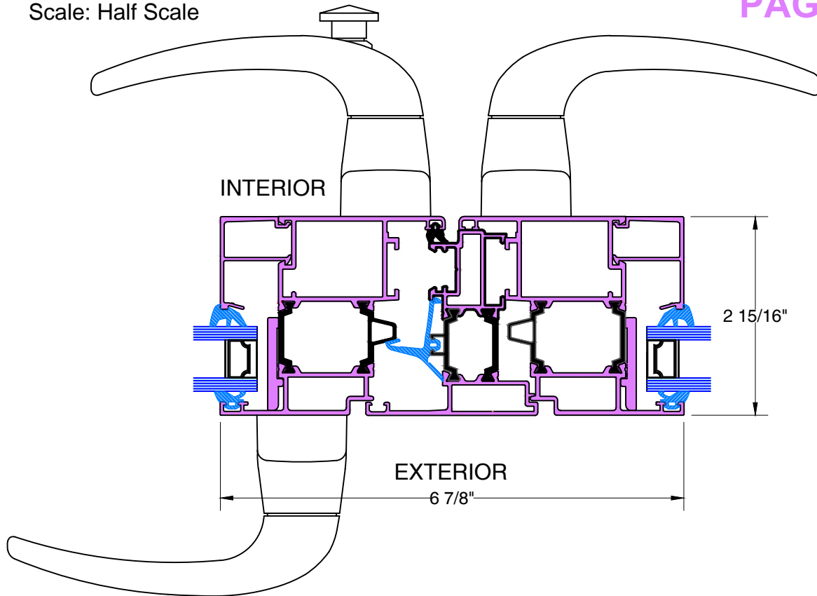
F TYPICAL FRENCH MEETING RAIL
