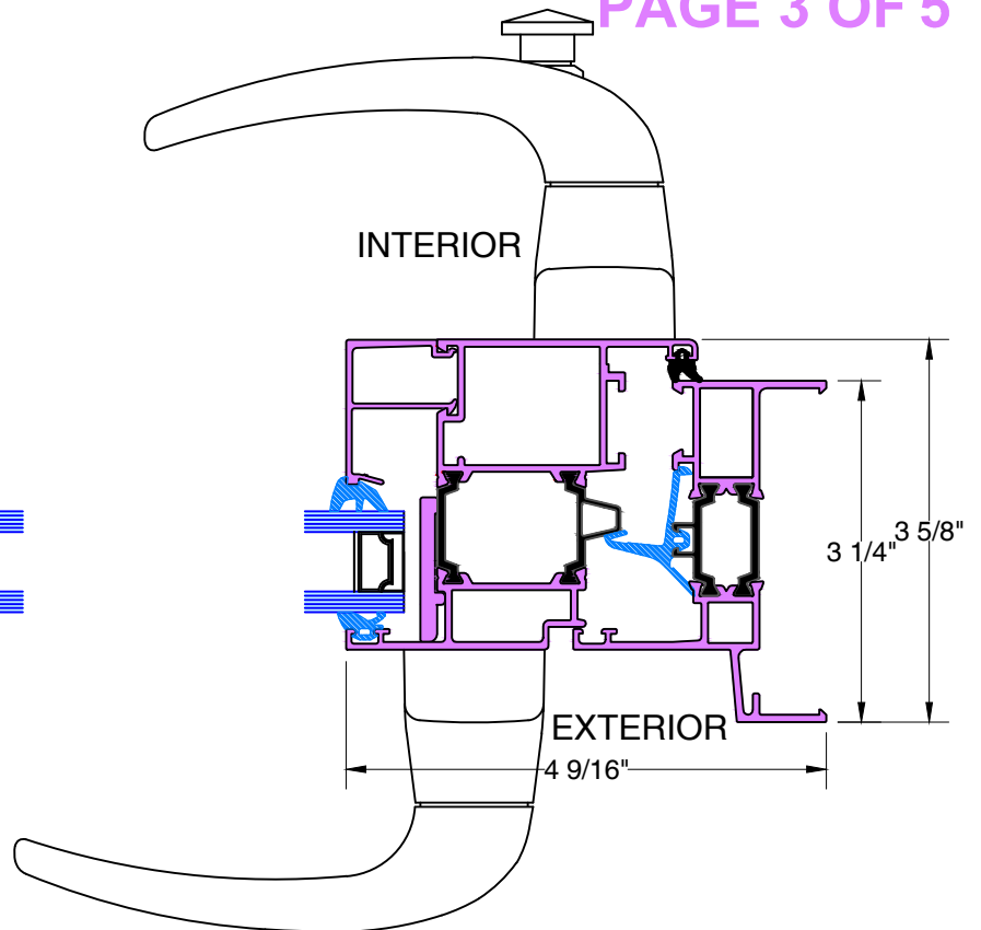
C TYPICAL LOCKING JAMB
