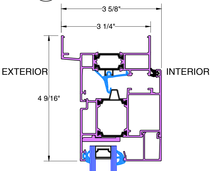
D TYPICAL HEAD
