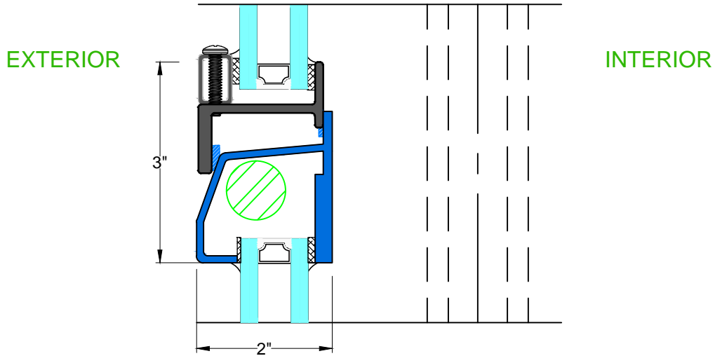
G TYPICAL LOUVER
