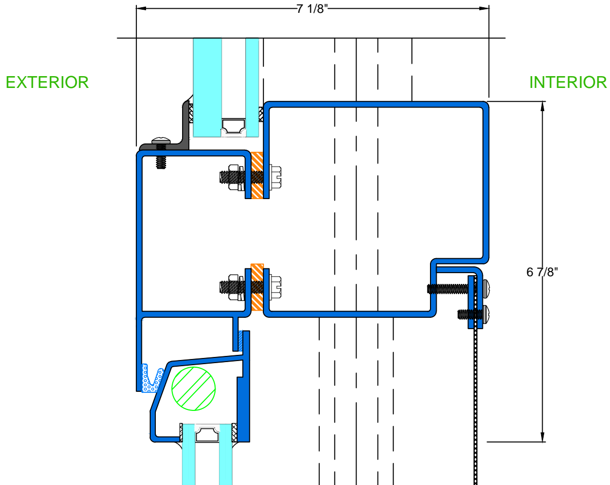
F TYPICAL MULLION
