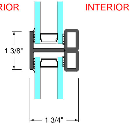
F TYPICAL HORIZONTAL MUNTIN
