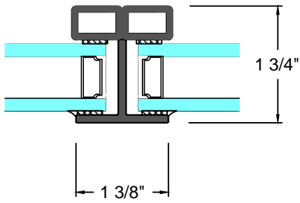
E TYPICAL VERTICAL MUNTIN
