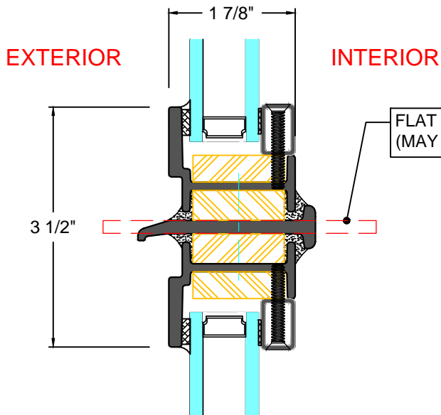
G TYPICAL STACKING MULLION
