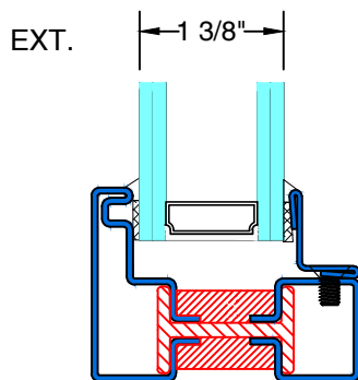
GB-2040 GLAZING BEAD
