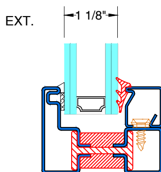
GB-1007 GLAZING BEAD
