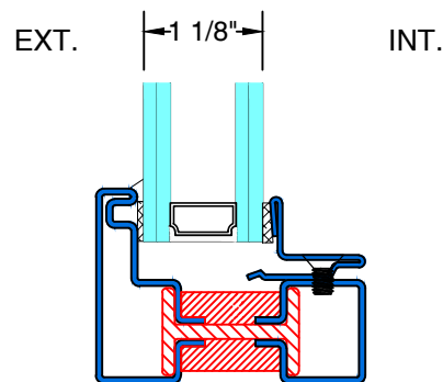
GB-2038 GLAZING BEAD
