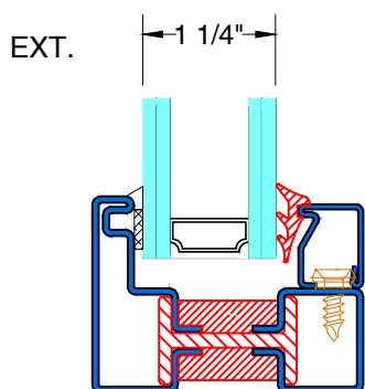
GB-2007 GLAZING BEAD
