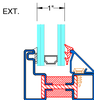
GB-1015 GLAZING BEAD
