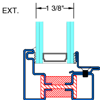
GB-2038 GLAZING BEAD
